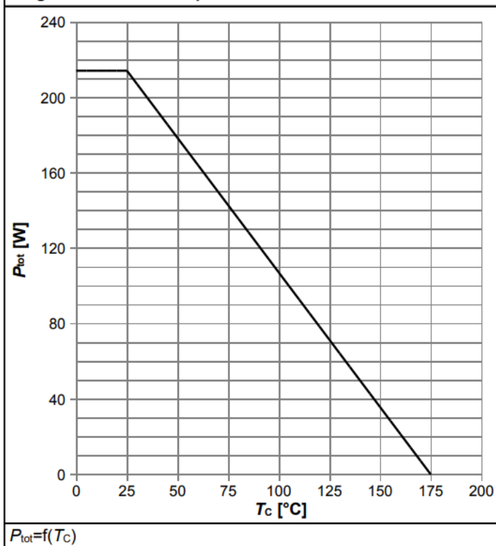
Diagram 1: Power dissipation
