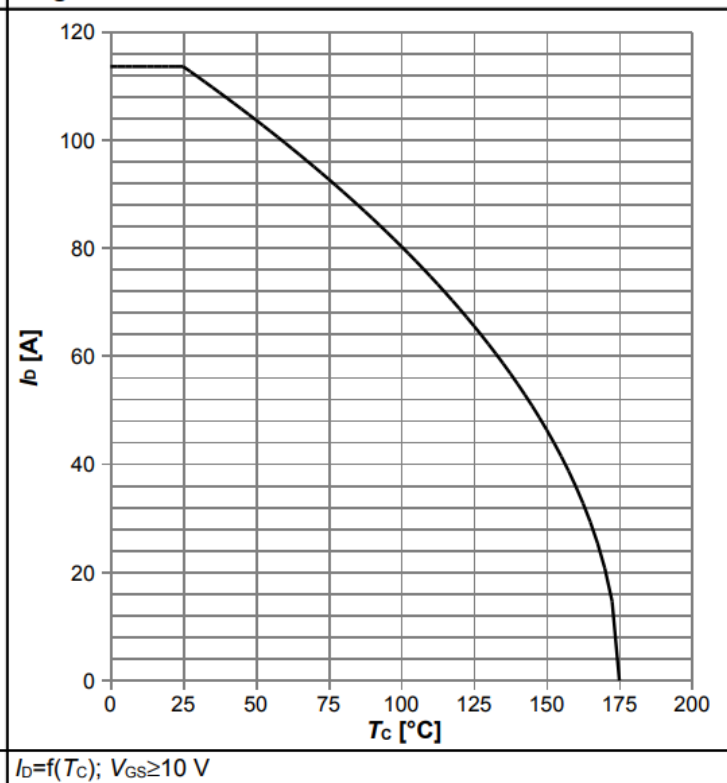
Diagram 2: Drain current
