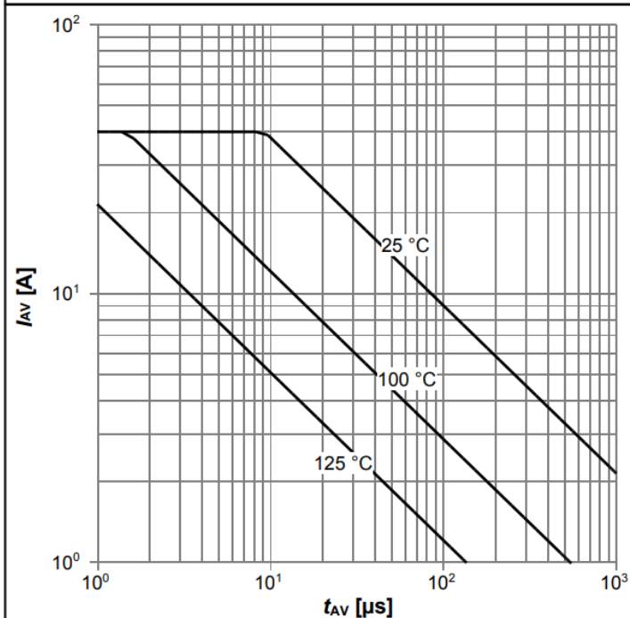
Diagram 13: Avalanche characteristics
