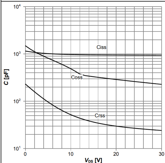
Diagram 11: Typ. capacitances
