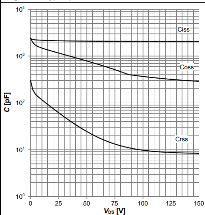
Diagram 11: Typ. capacitances
