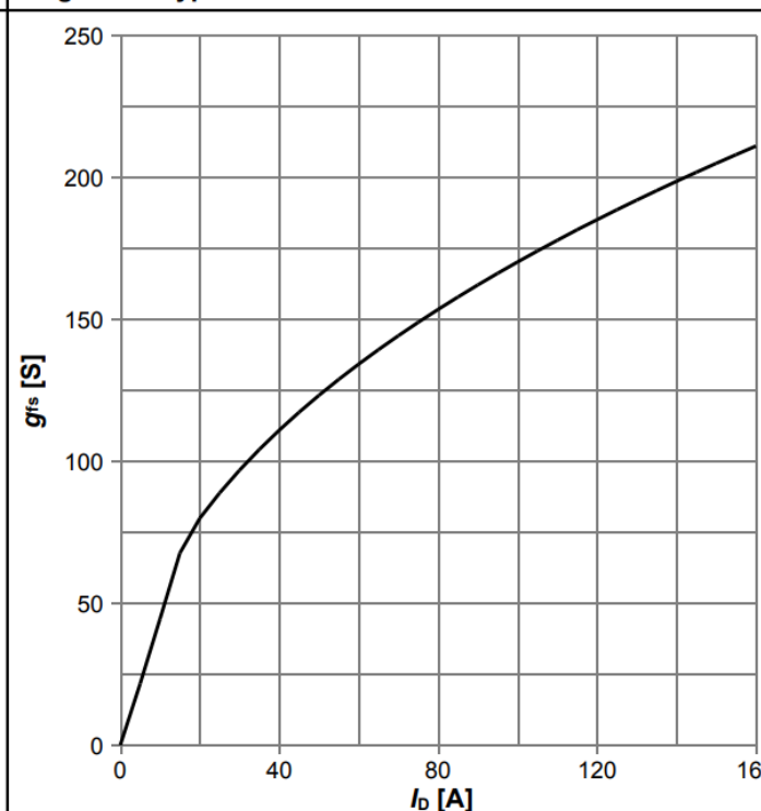
Diagram 8: Typ. forward transconductance
