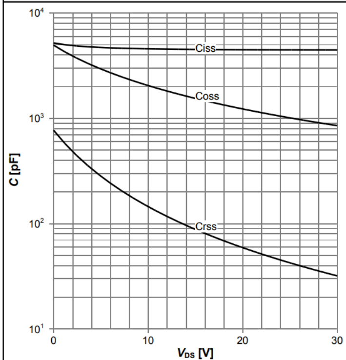
Diagram 11: Typ. capacitances
