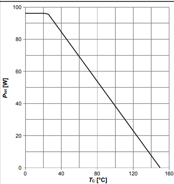
Diagram 1: Power dissipation
