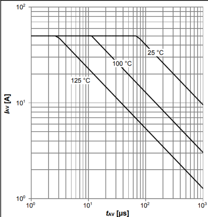
Diagram 13: Avalanche characteristics
