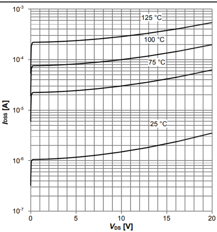
Diagram 15: Typ. drain-source leakage current
