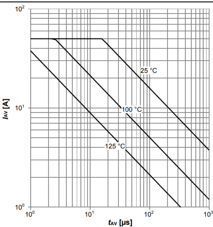
Diagram 13: Avalanche characteristics
