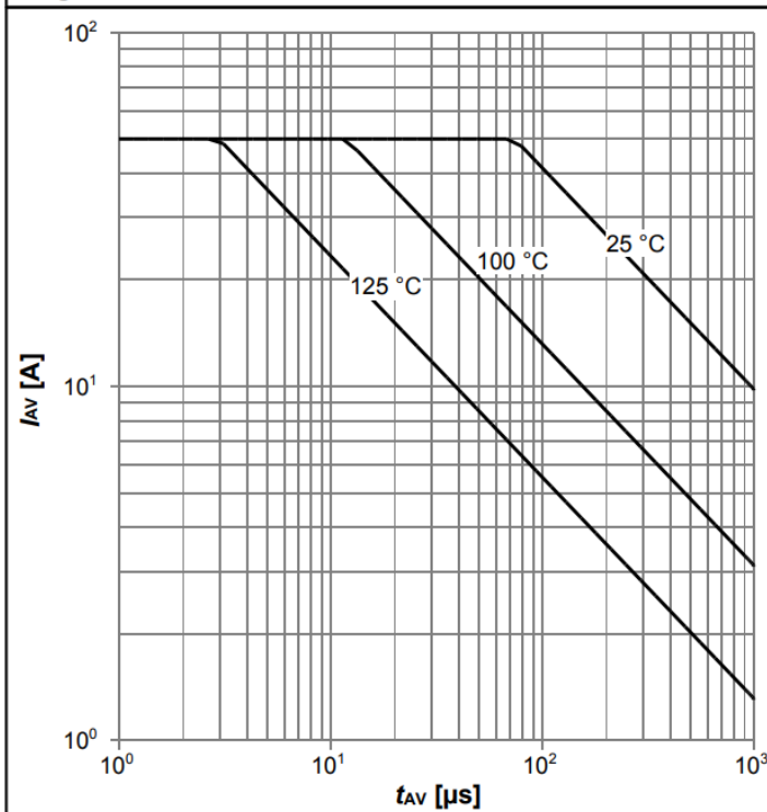
Diagram 13: Avalanche characteristics
