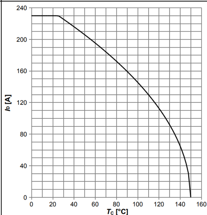
Diagram 2: Drain current
