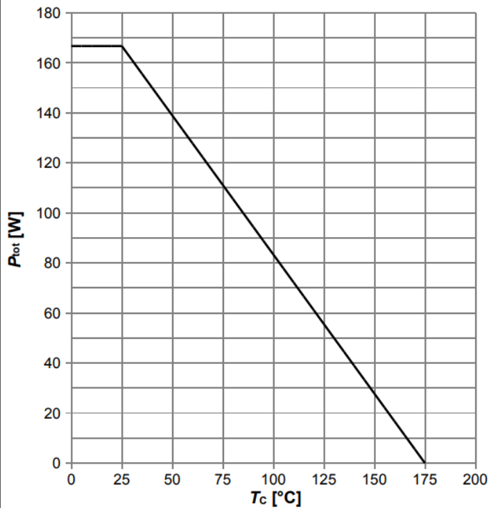
Diagram 1: Power dissipation
