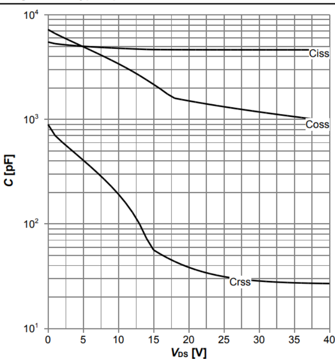
Diagram 11: Typ. capacitances
