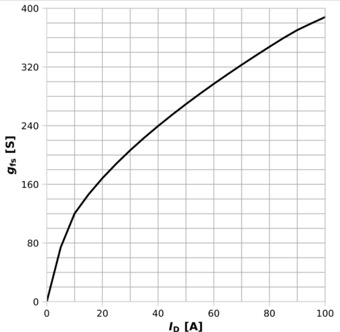
Diagram 8: Typ. forward transconductance
