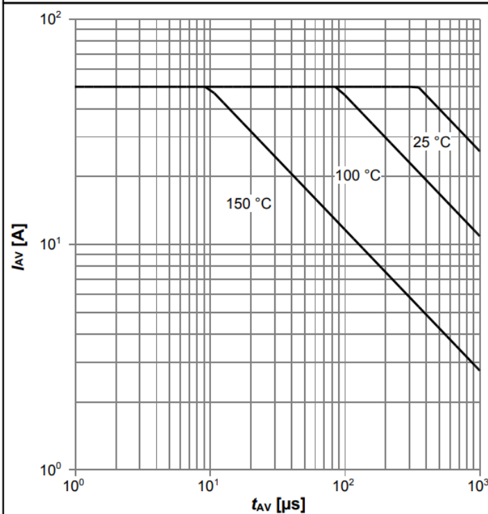
Diagram 13: Avalanche characteristics
