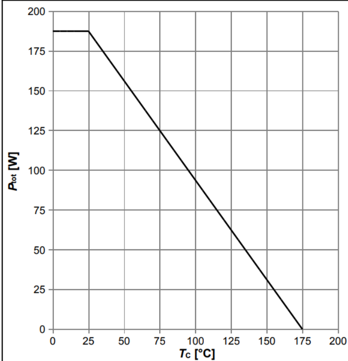
Diagram 1: Power dissipation
