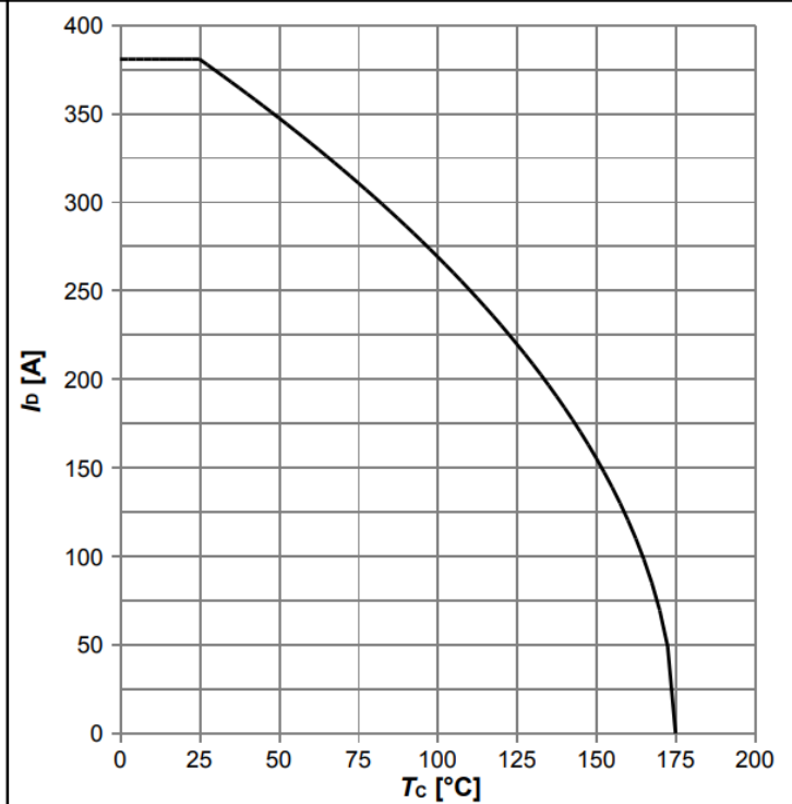
Diagram 2: Drain current
