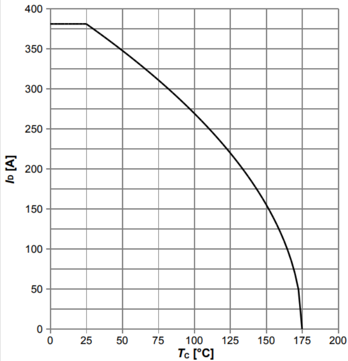
Diagram 2: Drain current
