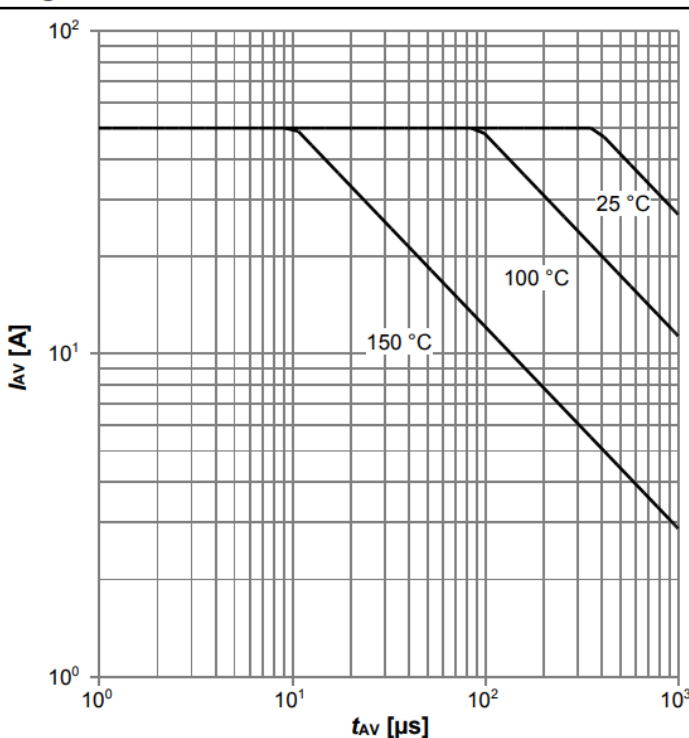
Diagram 13: Avalanche characteristics
