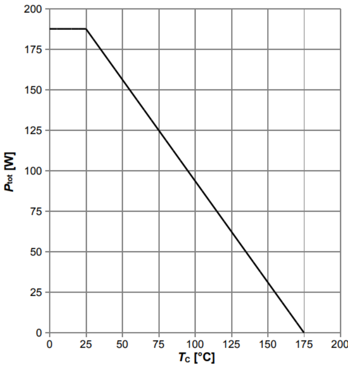
Diagram 1: Power dissipation
