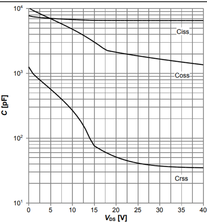
Diagram 11: Typ. capacitances
