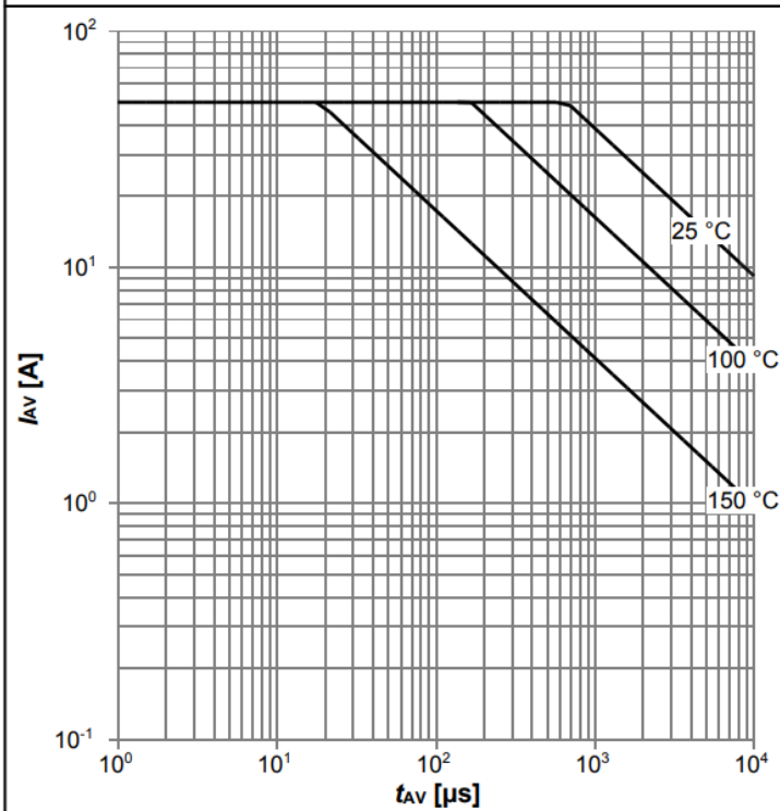
Diagram 13: Avalanche characteristics
