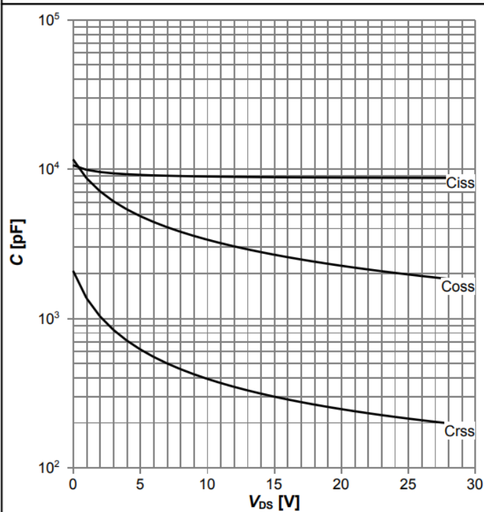
Diagram 11: Typ. capacitances
