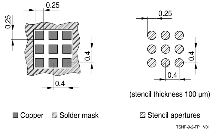
Figure 7: TSNP-9-2 Footprint Recommendation
