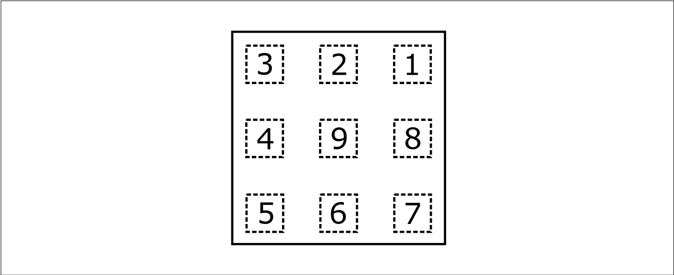
Figure 1: BGA10M1MN9 Pin Configuration (top view)
