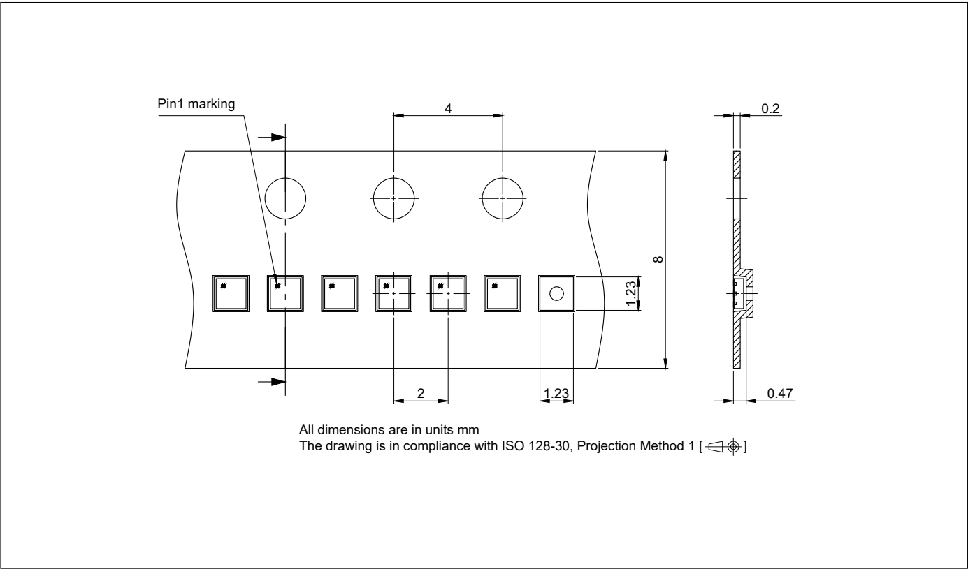
Figure 10: TSNP-9-6 Carrier Tape
