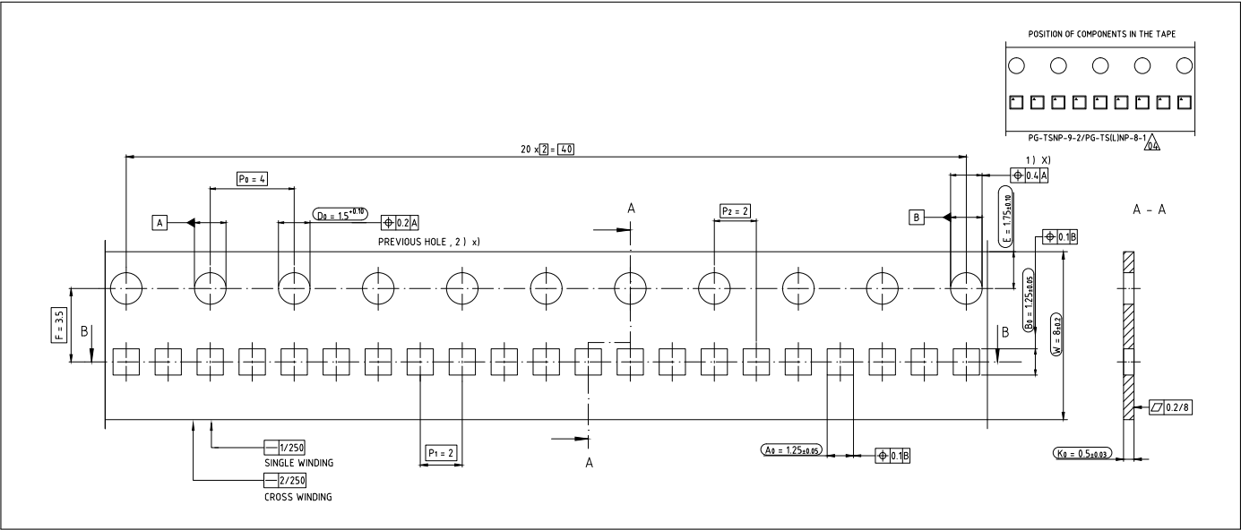
Figure 9: TSNP-9-2 Carrier Tape
