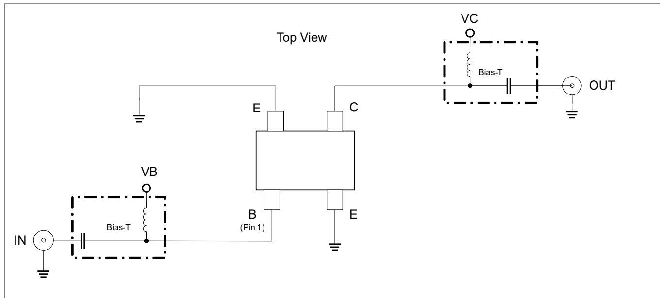
Figure 2 Testing circuit
