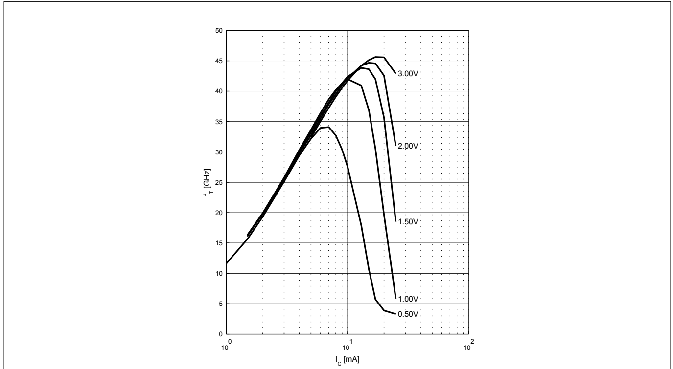
Figure 5 Transition frequency f_T = f(I_C, V_{CE}) , f = 1 GHz, V_{CE} = \text{parameter}
