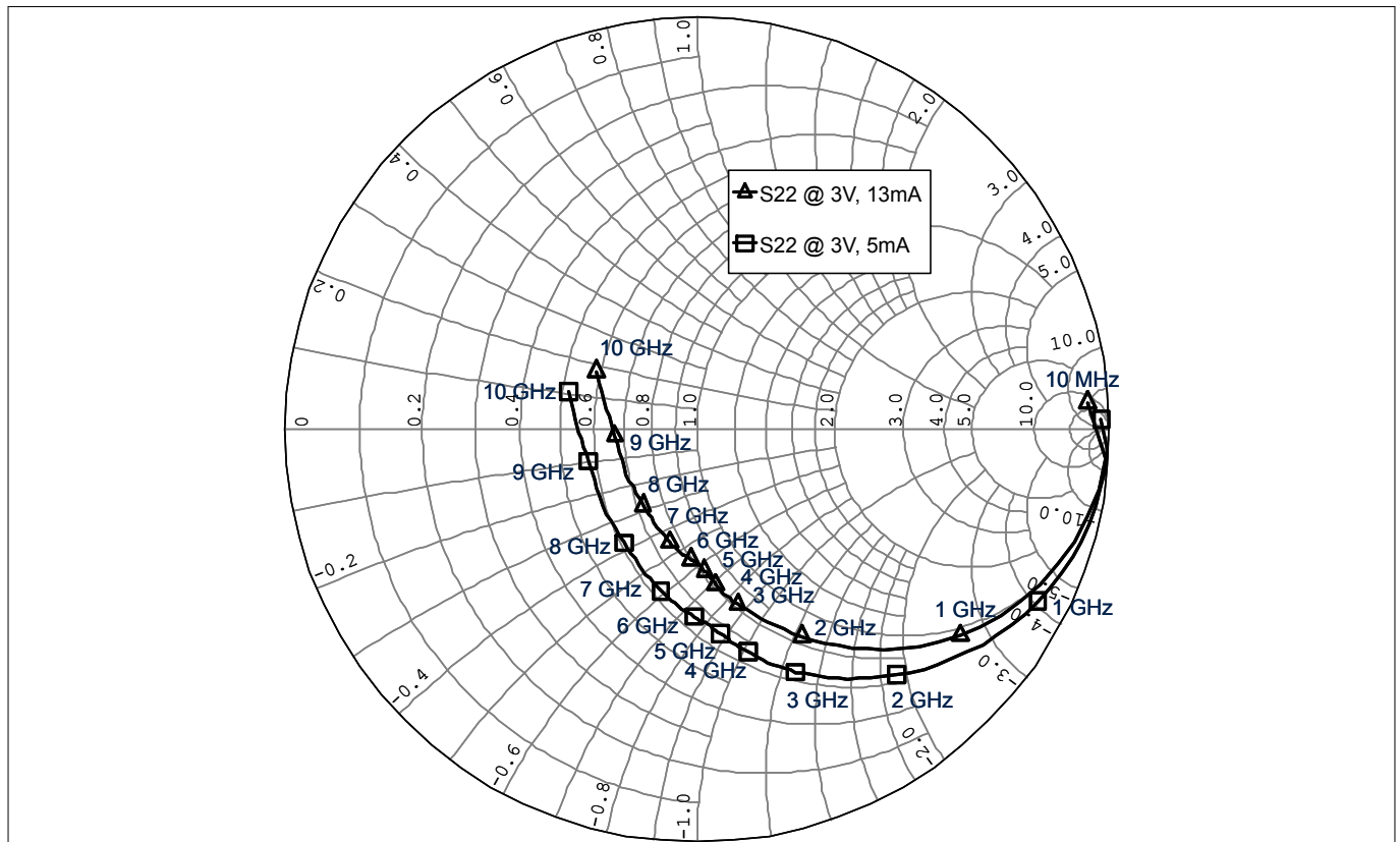
Figure 10 Output reflection coefficient S_{22} = f(f) , V_{CE} = 3V , I_C = 5 / 13mA
