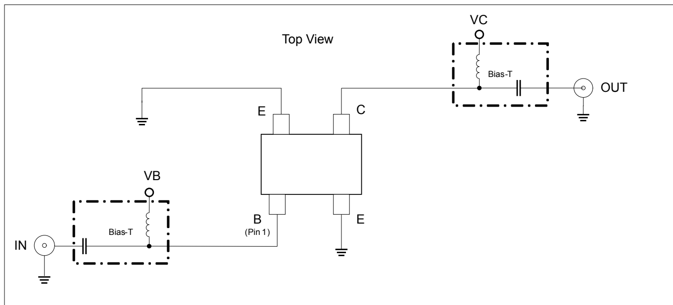
Figure 4 Testing circuit
