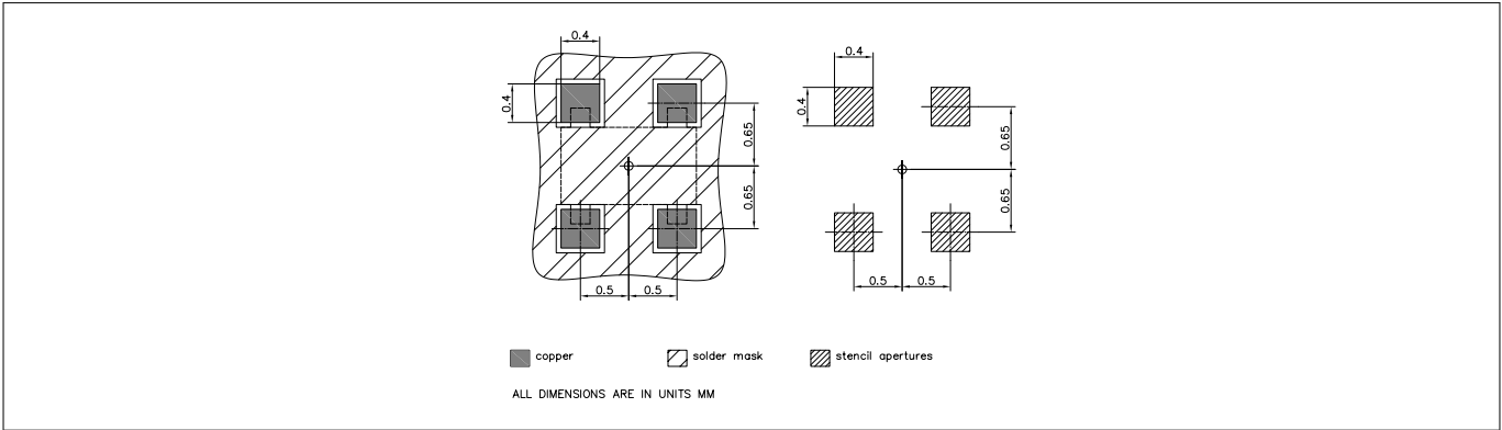
Figure 15 Foot print
