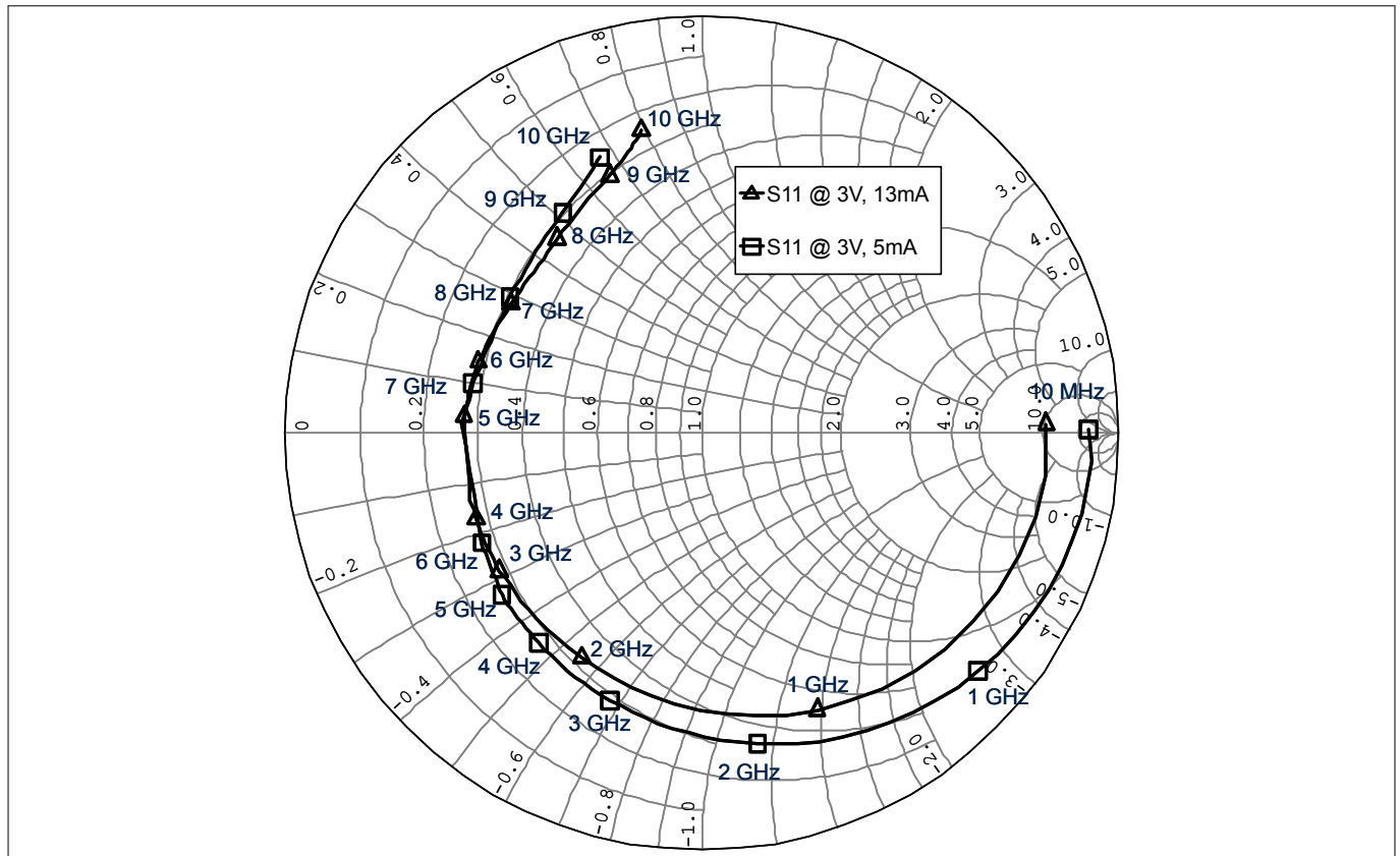
Figure 9 Input reflection coefficient S_{11} = f(f) , V_{CE} = 3V , I_C = 5 / 13mA
