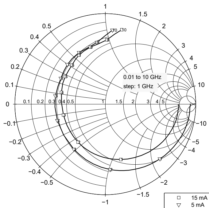
Figure 14 Input reflection coefficient S_{11} = f(f) , V_{CE} = 3 \text{ V} , I_C = 5 / 15 \text{ mA}
