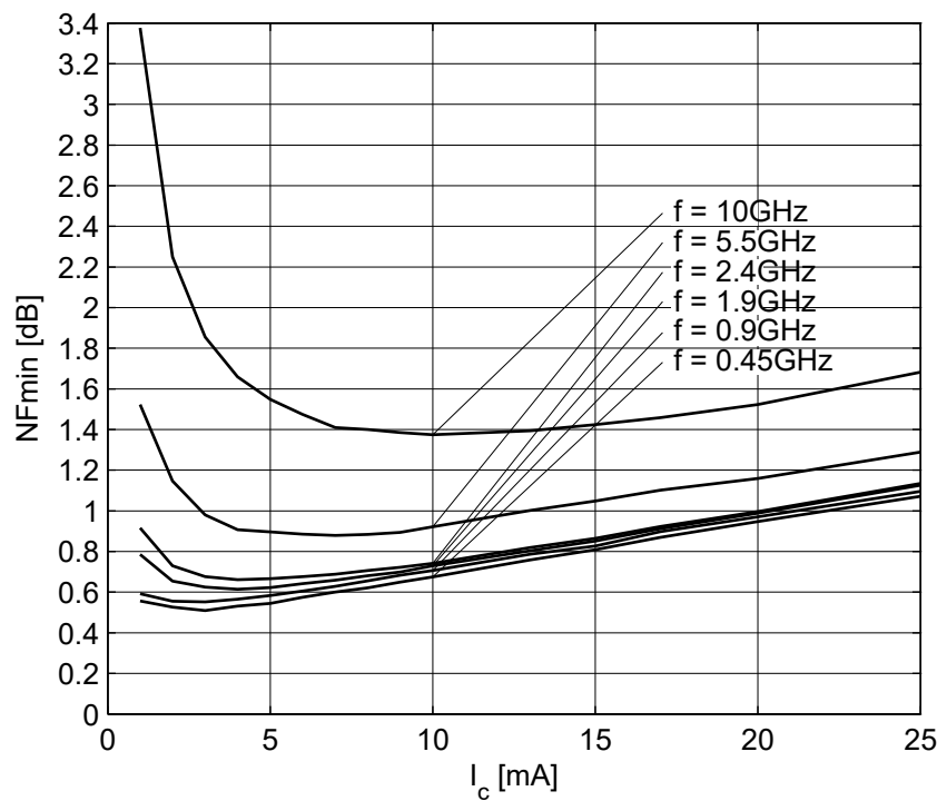
Figure 18 Noise figure NF_{min} = f(I_c) , V_{CE} = 3\text{ V} , Z_S = Z_{S,opt} , f = \text{parameter in GHz}
