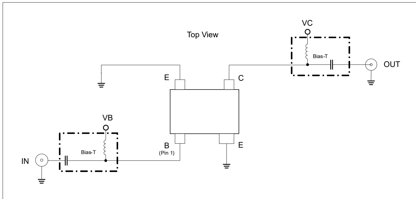
Figure 2 Testing circuit
