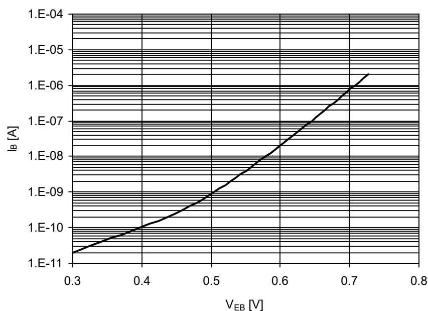
Figure 7 Base current vs. base emitter reverse voltage I_B = f(V_{EB}) , V_{CE} = 2 V
