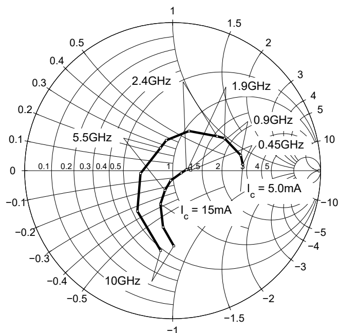
Figure 15 Source impedance for minimum noise figure Z_{s,opt} = f(f) , V_{CE} = 3 \text{ V} , I_C = 5 / 15 \text{ mA}
