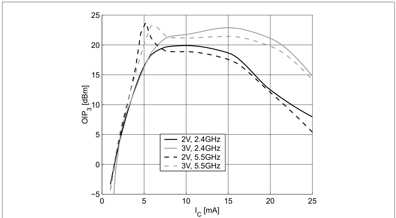
Figure 9 3rd order intercept point at output OIP_3 [dBm] = f(I_C) , Z_S = Z_L = 50 \Omega , V_{CE} , f = \text{parameters}
