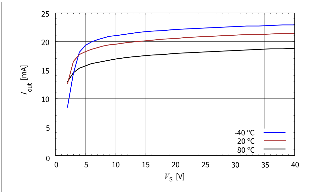
图 3-7 输出电流与 V_S I_{out} = f(V_S) , V_S - V_{out} = 1.4 \text{ V} , T_A = \text{Parameter}
