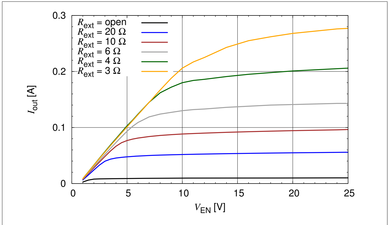
Figure 3-12 BCR 320U: Output Current versus V_{EN} I_{out} = f(V_{EN}) , V_{out} = 2 V, R_{ext} = Parameter
