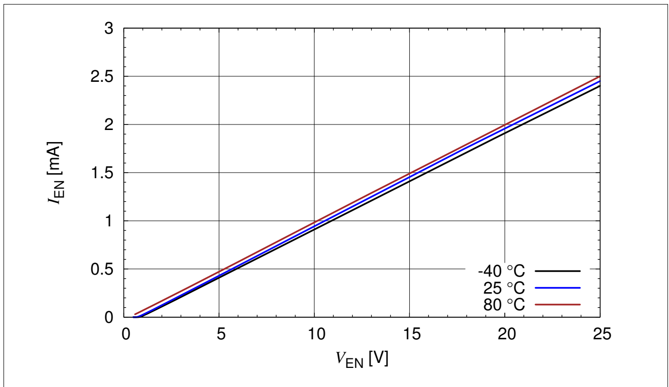
Figure 3-13 BCR 320U: Enable Current versus V_{EN} I_{EN} = f(V_{EN}) , R_{ext} = \text{open} , I_{out} = 0 A, T_A = Parameter
