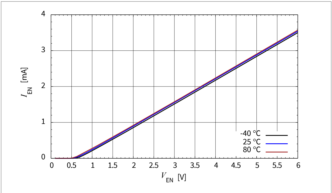
图 3-23 BCR 321U: 使能电流与 V_{EN} I_{EN} = f(V_{EN}), R_{ext} = \text{open}, I_{out} = 0 \text{ A}, T_A = \text{Parameter}
