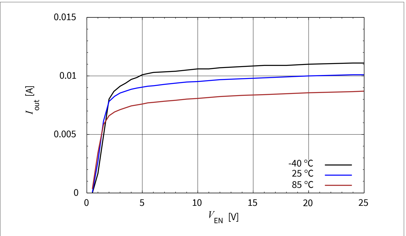
图 3-9 BCR 320U: 输出电流与 V_{EN} I_{out} = f(V_{EN}), V_{out} = 2\text{ V}, R_{ext} = \text{open}, T_A = \text{Parameter}
