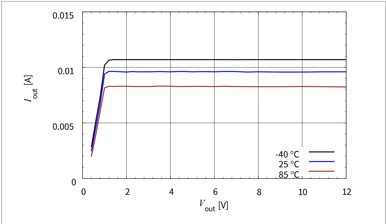
图3-16 BCR 321U: 输出电流与 V_{out} I_{out} = f(V_{out}) , V_{EN} = 3.3\text{ V} , R_{ext} = \text{open} , T_A = \text{Parameter}
