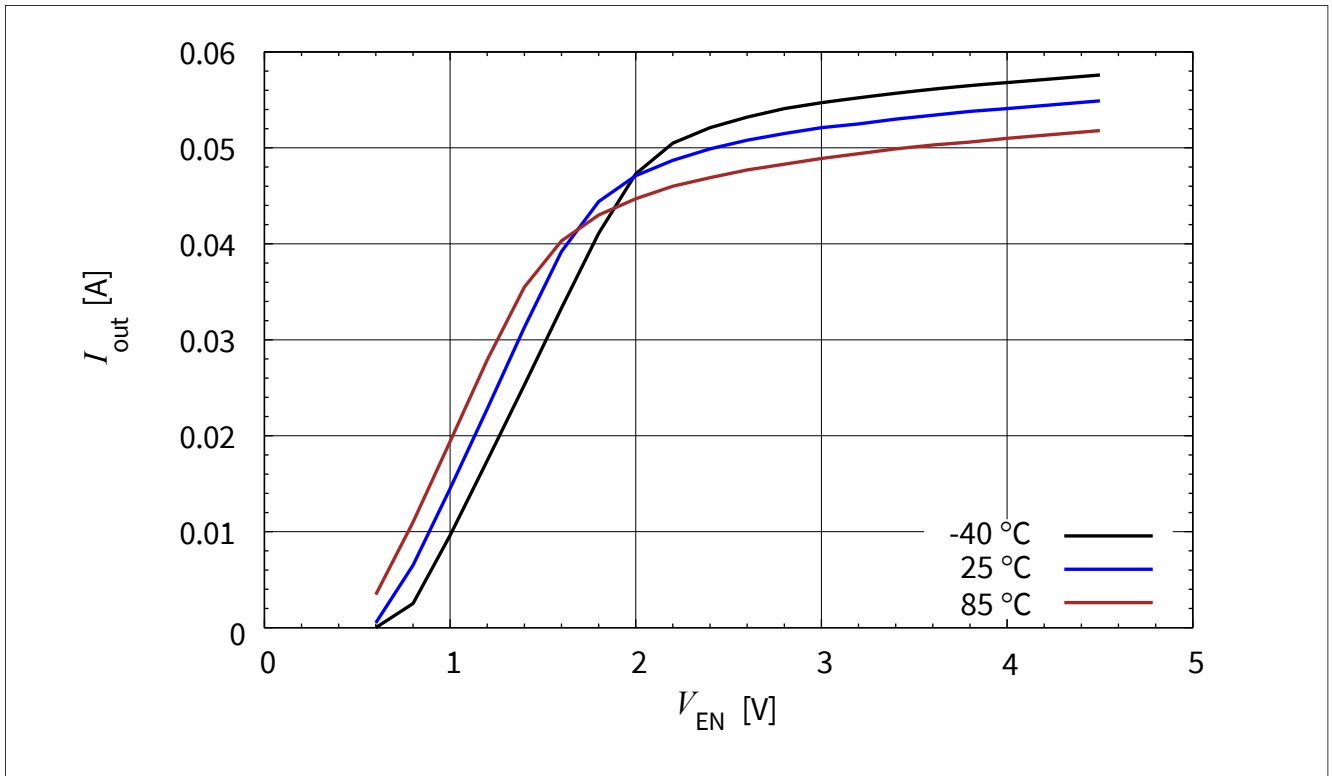
图 3-20 BCR 321U: 输出电流与 V_{EN} I_{out} = f(V_{EN}), V_{out} = 2\text{ V}, R_{ext} = 20\ \Omega, T_A = \text{Parameter}
