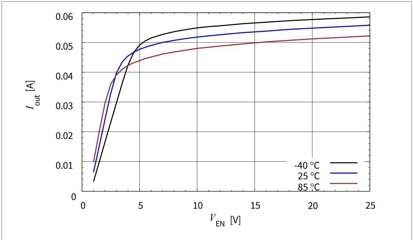
图3-10 BCR 320U: 输出电流与 V_{EN} I_{out} = f(V_{EN}) , V_{out} = 2\text{ V} , R_{ext} = 20\ \Omega , T_A = \text{Parameter}
