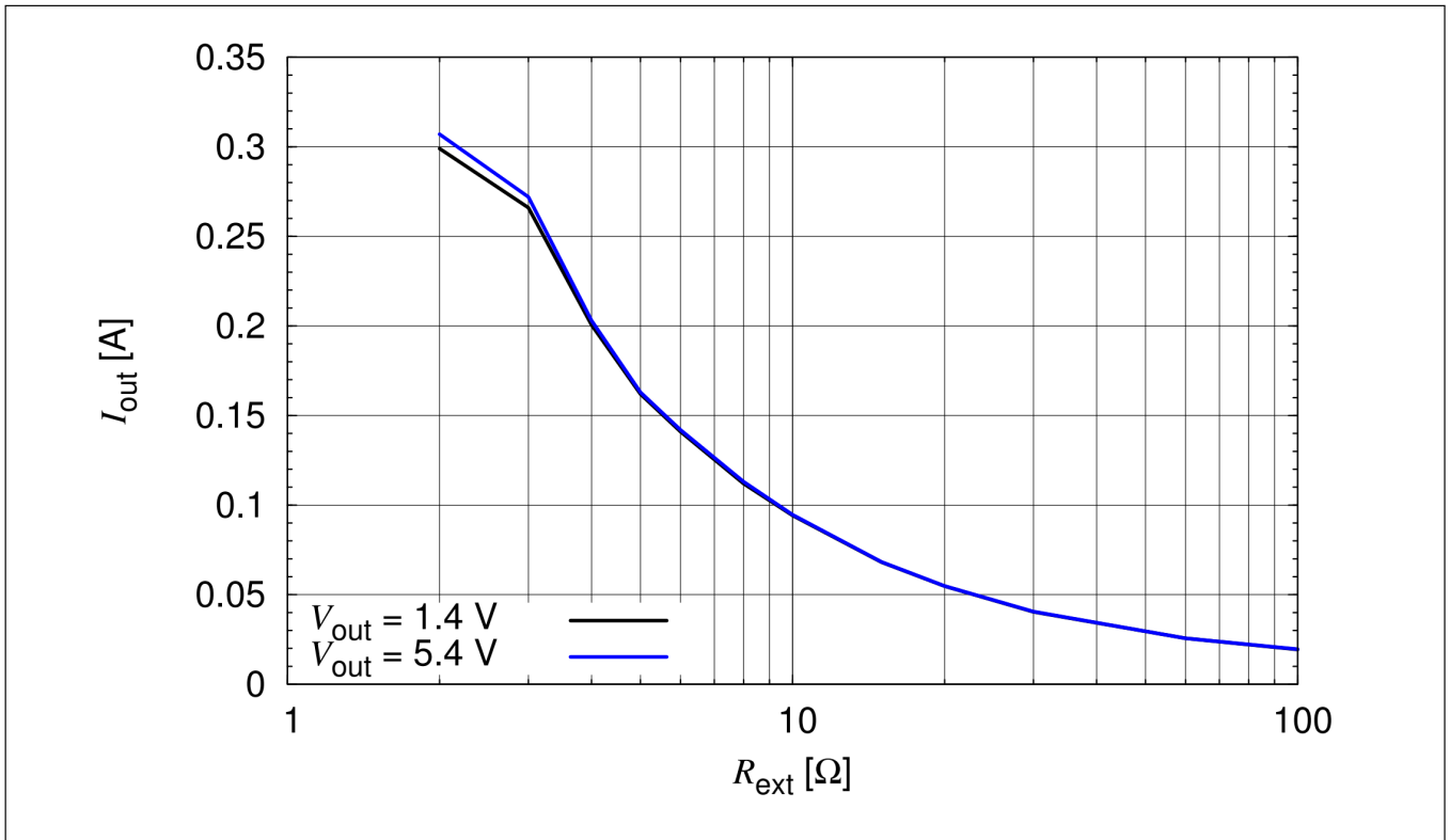
图 3-5 BCR 320U: 输出电流 R_{ext} I_{out} = f(R_{ext}), V_{EN} = 12 V, V_{out} = \text{Parameter}
