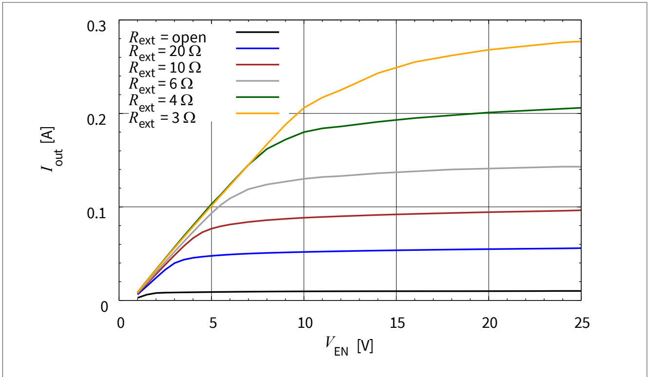
图 3-12 BCR 320U: 输出电流与 V_{EN} I_{out} = f(V_{EN}), V_{out} = 2 V, R_{ext} = \text{Parameter}
