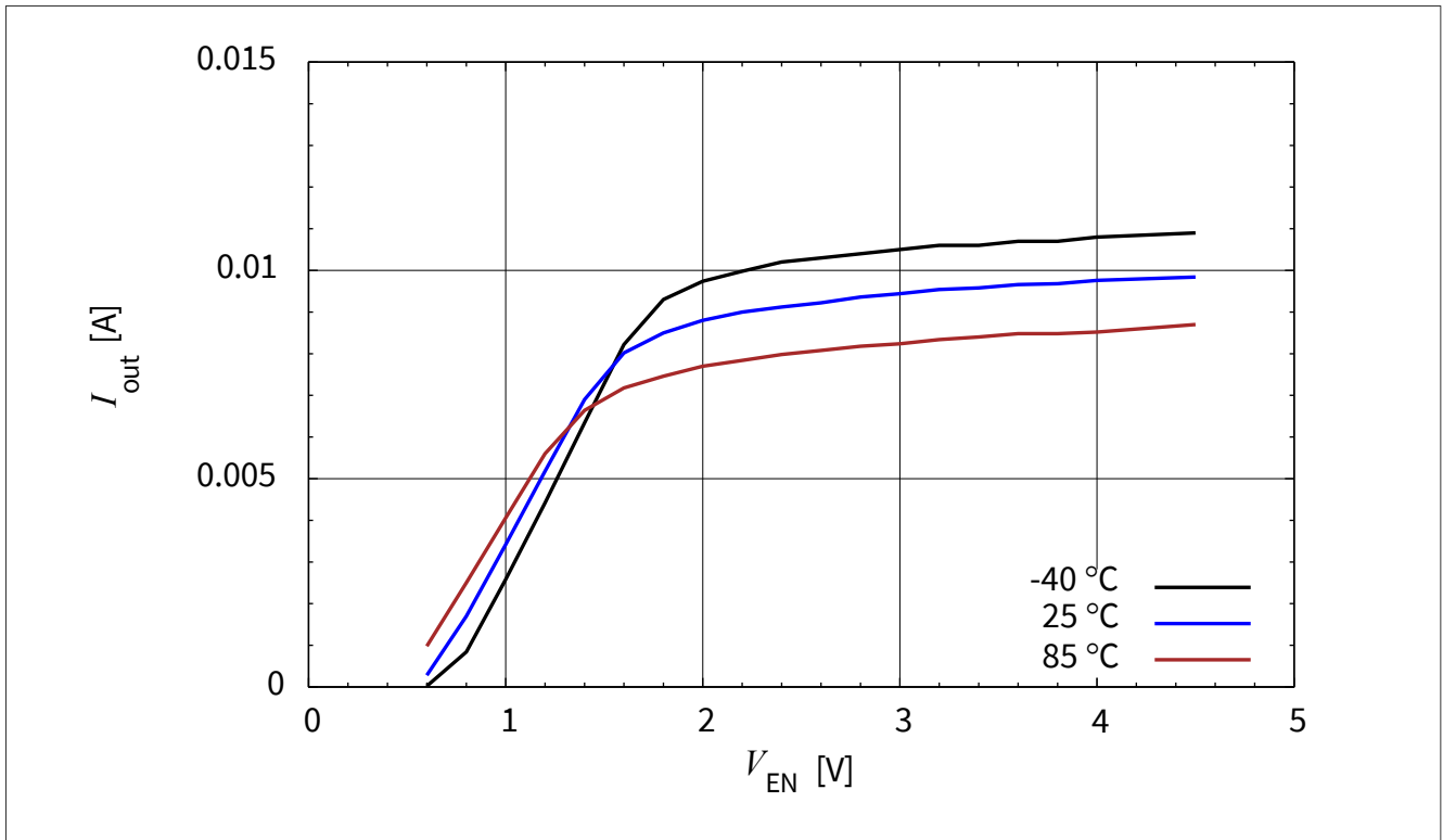
图 3-19 BCR 321U: 输出电流与 V_{EN} I_{out} = f(V_{EN}), V_{out} = 2\text{ V}, R_{ext} = \text{open}, T_A = \text{Parameter}
