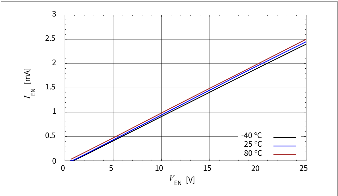
图 3-13 BCR 320U: 使能电流与 V_{EN} I_{EN} = f(V_{EN}), R_{ext} = \text{open}, I_{out} = 0 A, T_A = \text{Parameter}
