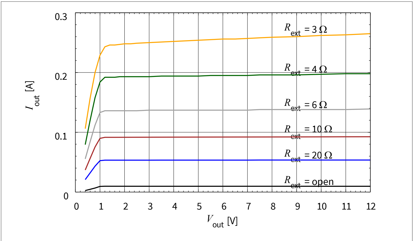
图 3-14 BCR 321U: 输出电流与 V_{out} I_{out} = f(V_{out}), V_{EN} = 3.3\text{ V}, R_{ext} = \text{Parameter}
