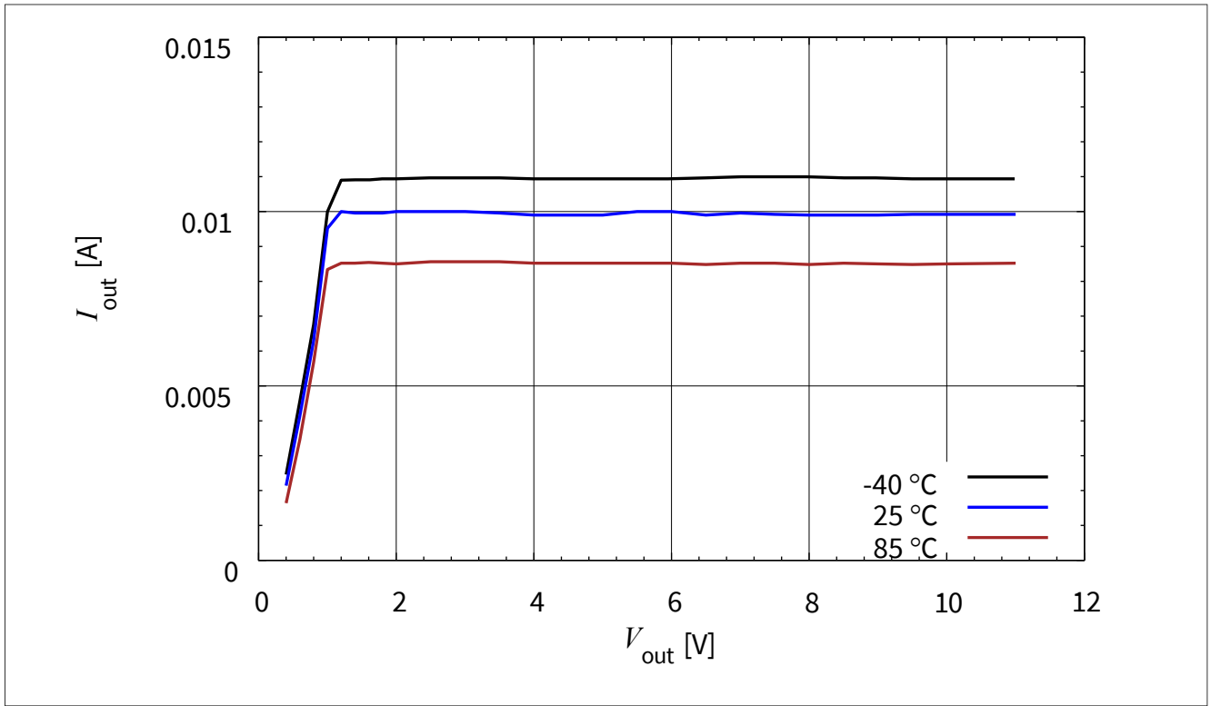
图 3-6 BCR 320U: 输出电流与 V_{out} I_{out} = f(V_{out}), V_{EN} = 12\text{ V}, R_{ext} = \text{open}, T_A = \text{Parameter}
