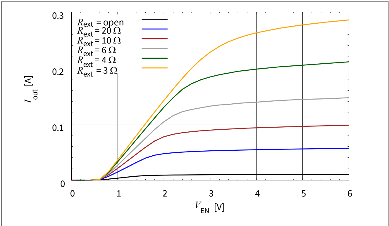
图 3-22 BCR 321U: 输出电流与 V_{EN} I_{out} = f(V_{EN}), V_{out} = 2 \text{ V}, R_{ext} = \text{Parameter}
