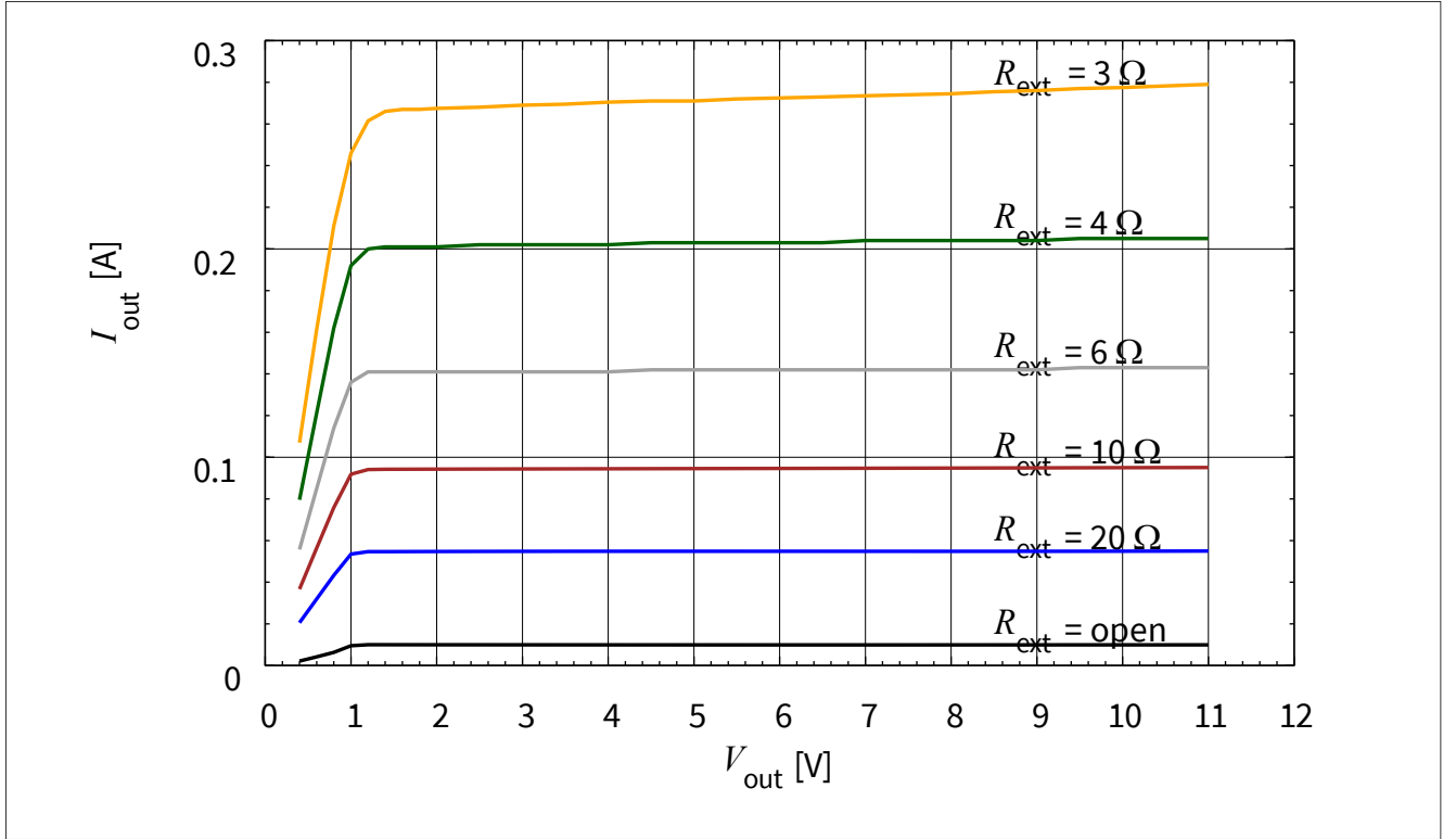
图 3-4 BCR 320U: 输出电流与 V_{out} I_{out} = f(V_{out}), V_{EN} = 12 V, R_{ext} = \text{Parameter}
