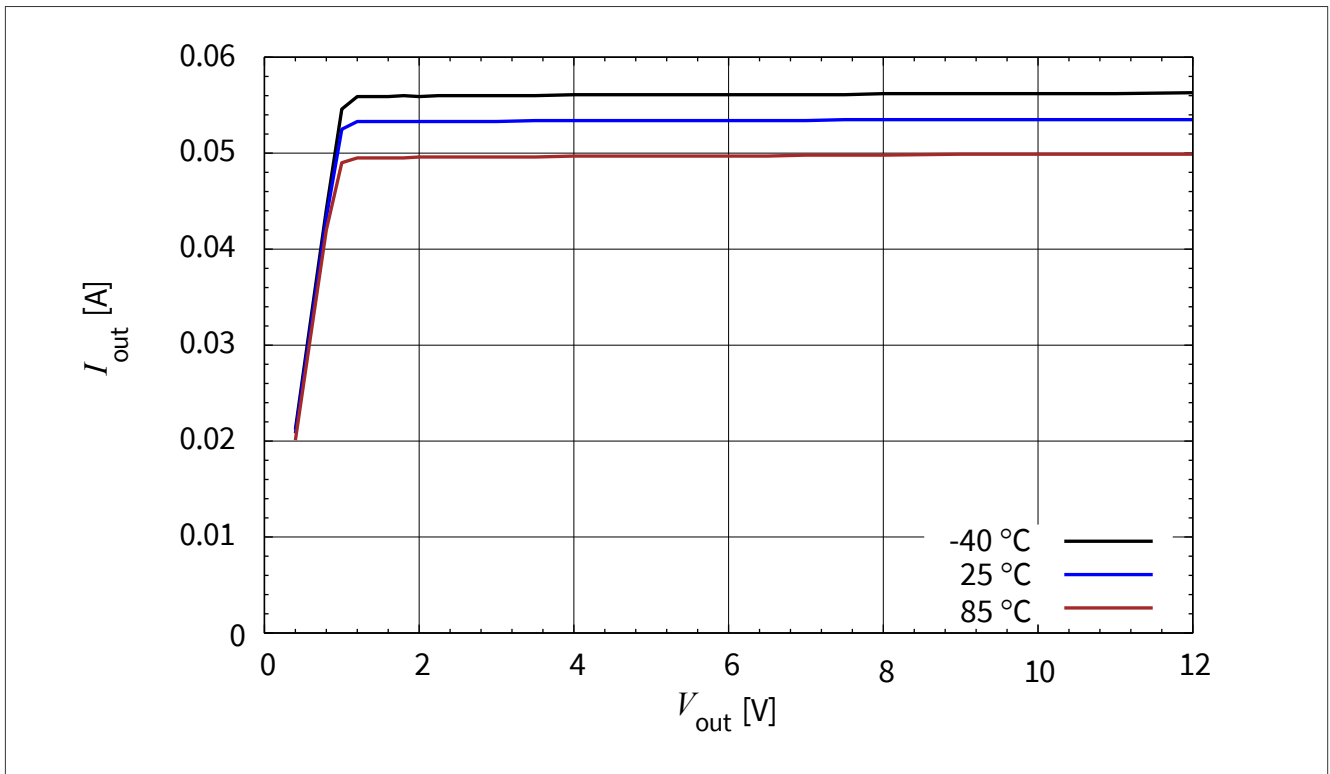
图 3-17 BCR 321U: 输出电流与 V_{out} I_{out} = f(V_{out}) , V_{EN} = 3.3\text{ V} , R_{ext} = 20\ \Omega , T_A = \text{Parameter}
