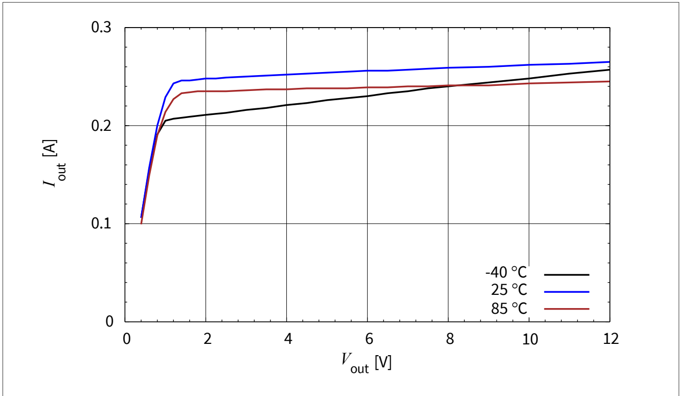
图 3-18 BCR 321U: 输出电流与 V_{out} I_{out} = f(V_{out}), V_{EN} = 3.3\text{ V}, R_{ext} = 3\ \Omega, T_A = \text{Parameter}
