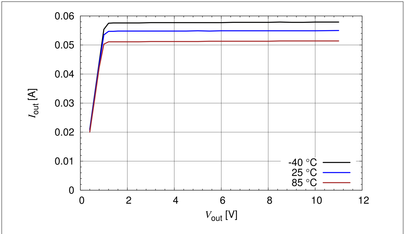
图 3-7 BCR 320U: 输出电流与 V_{out} I_{out} = f(V_{out}), V_{EN} = 12\text{ V}, R_{ext} = 20\ \Omega, T_A = \text{Parameter}
