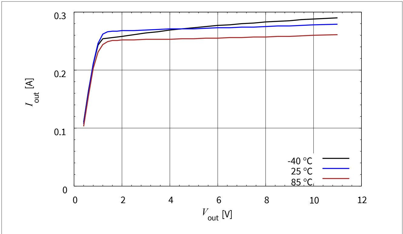
图 3-8 BCR 320U: 输出电流与 V_{out} I_{out} = f(V_{out}), V_{EN} = 12\text{ V}, R_{ext} = 3\ \Omega, T_A = \text{Parameter}
