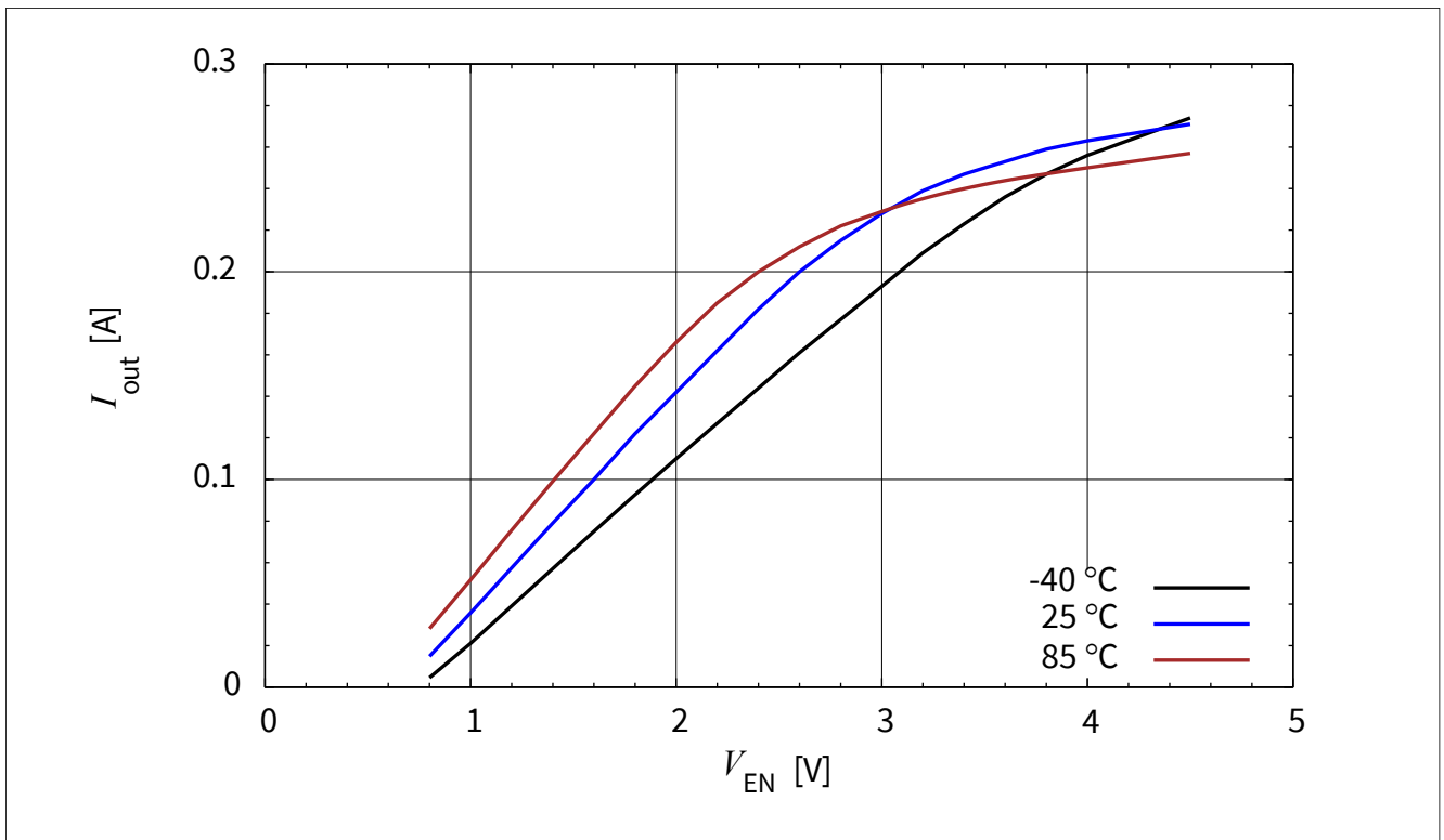
图 3-21 BCR 321U: 输出电流与 V_{EN} I_{out} = f(V_{EN}), V_{out} = 2\text{ V}, R_{ext} = 3\ \Omega, T_A = \text{Parameter}
