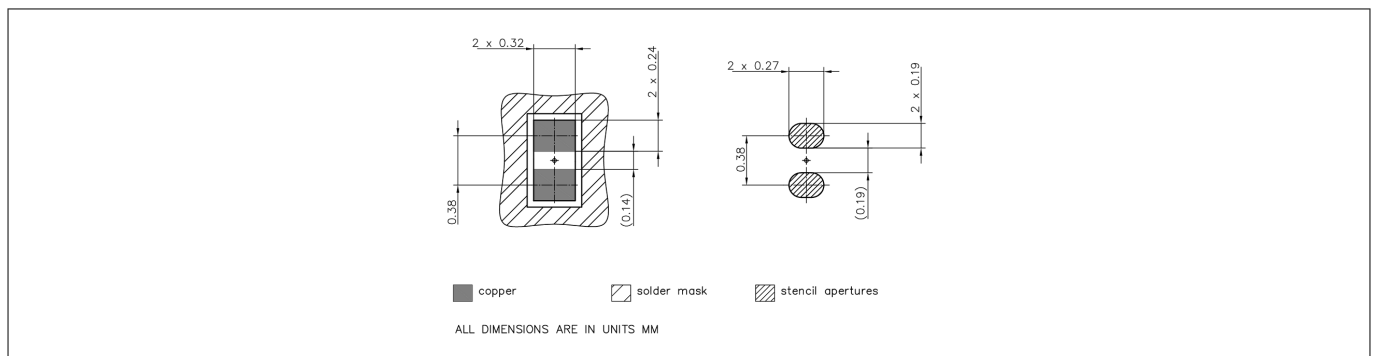
Figure 11 Foot print
