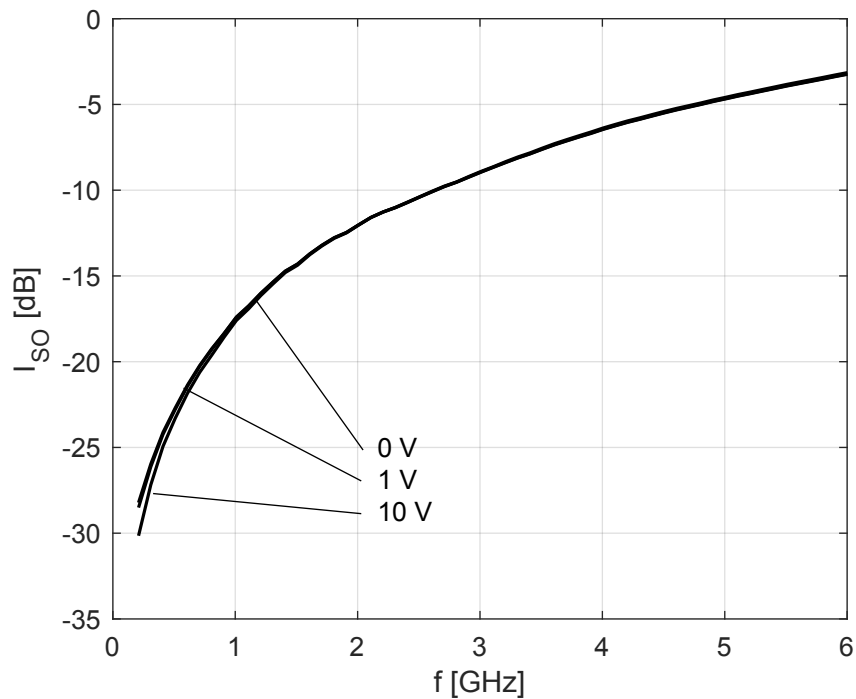
Figure 6 Isolation I_{S0} vs. frequency f at different reverse voltages
