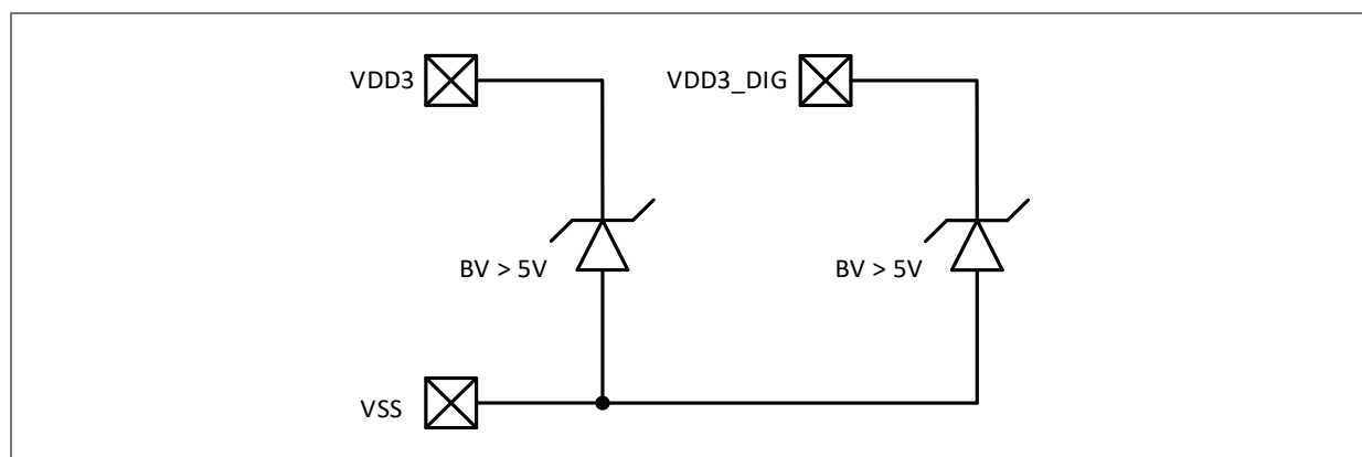
Figure 4: ESD protection circuit on VDD3 domain
