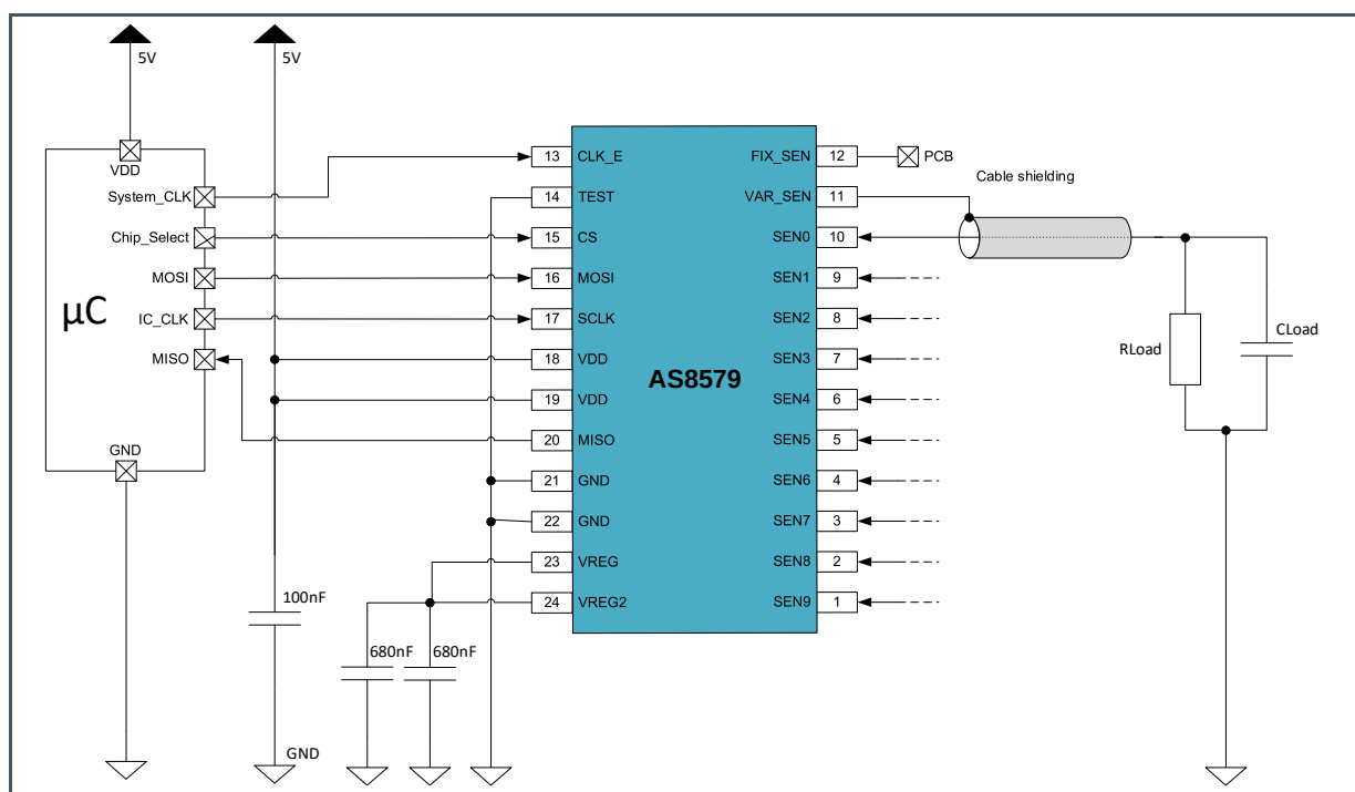
Figure 48: Typical Application Circuit
