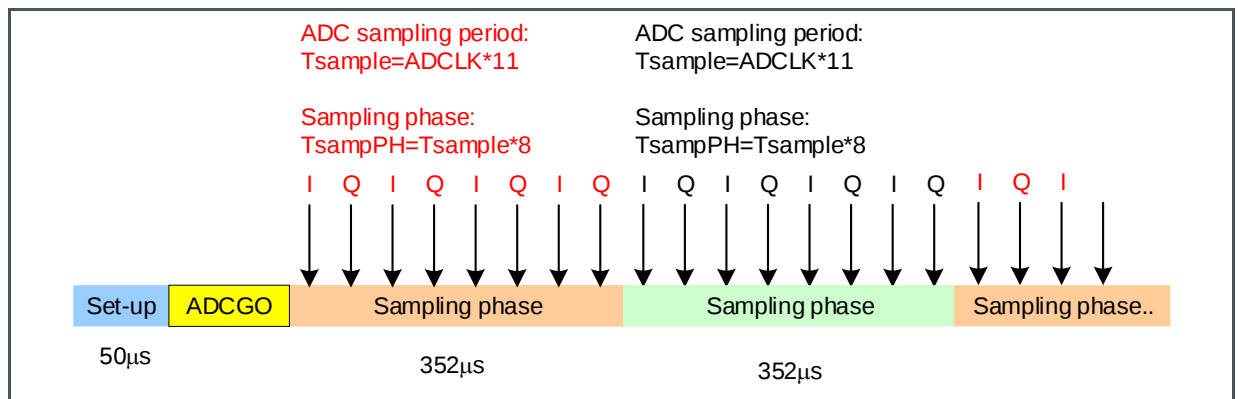
Figure 19: Measuring Cycle
