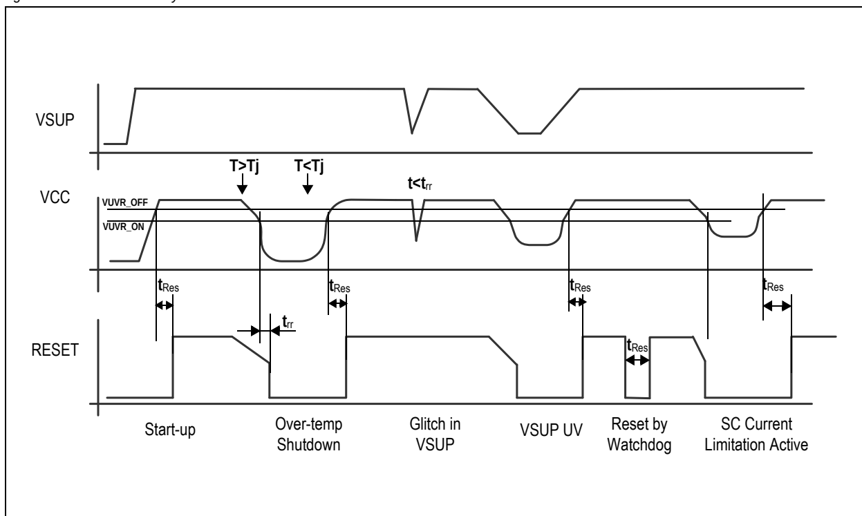
Figure 6. Reset Functionality
