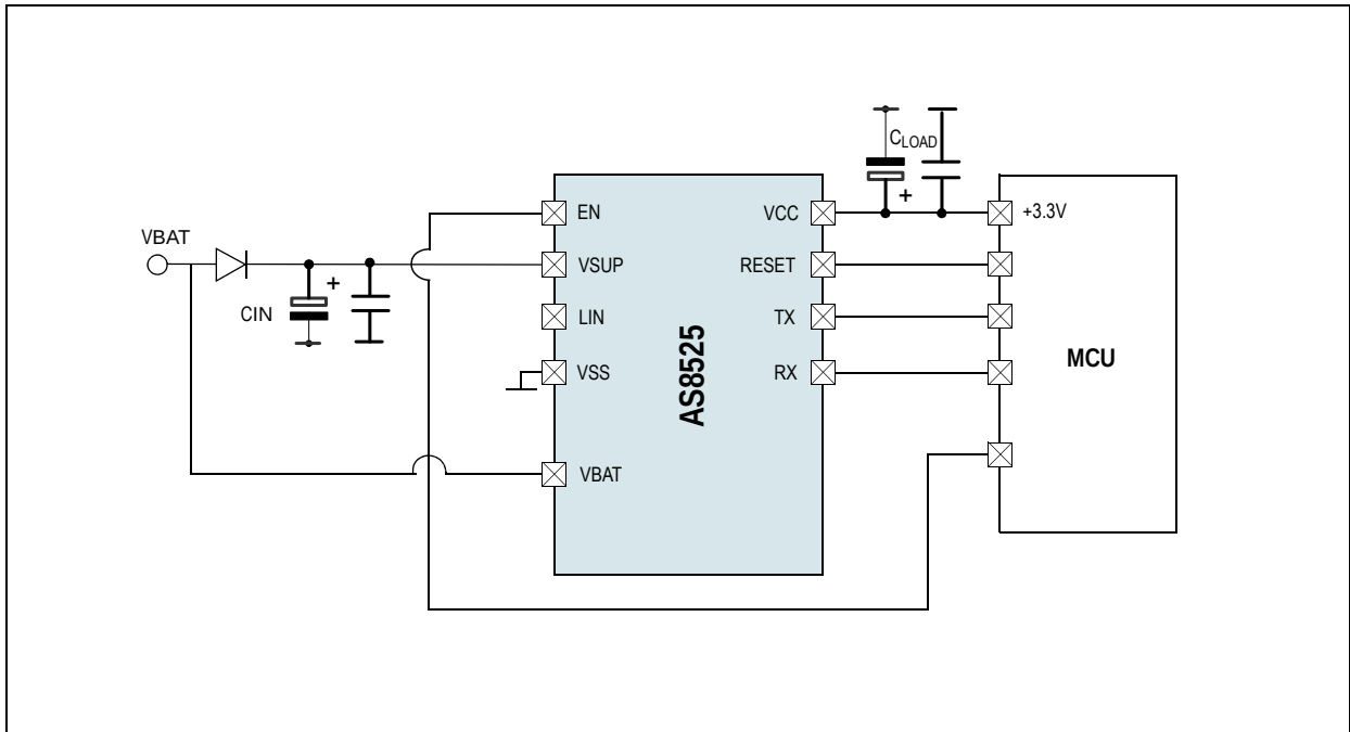
Figure 14. Enable Interface
