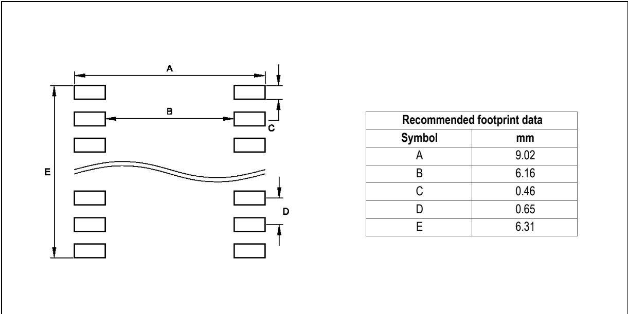
Figure 22: PCB footprint
