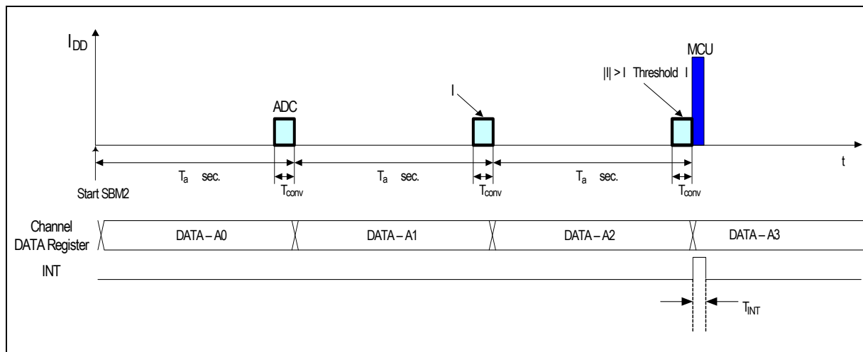
Figure 9: Standby mode2
