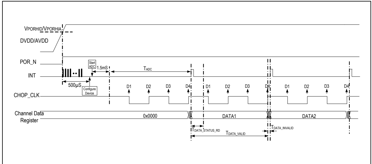
Figure 17: AS8512 device initialization sequence at power ON
