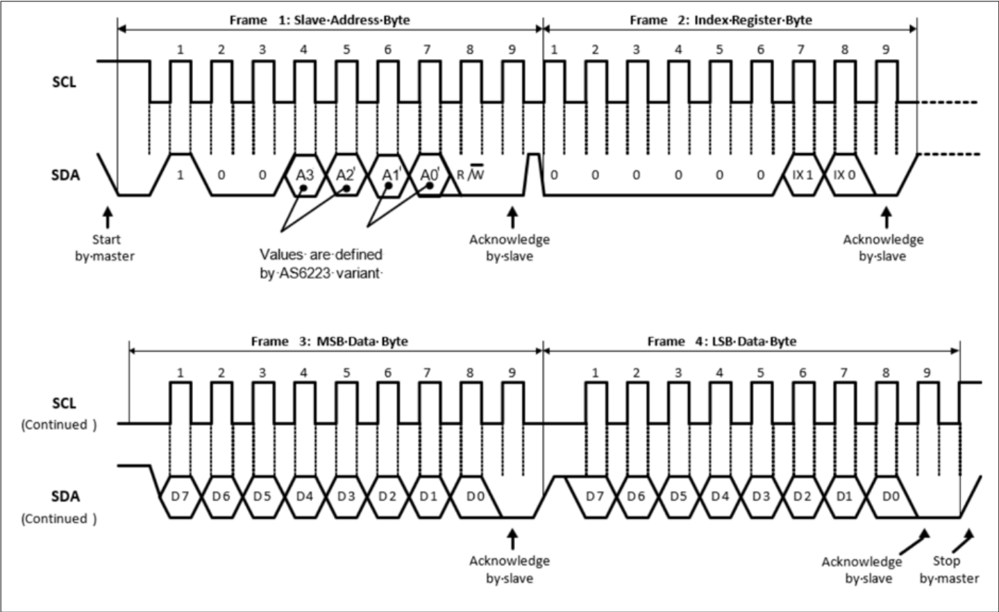
Figure 7 Timing diagram for word write
