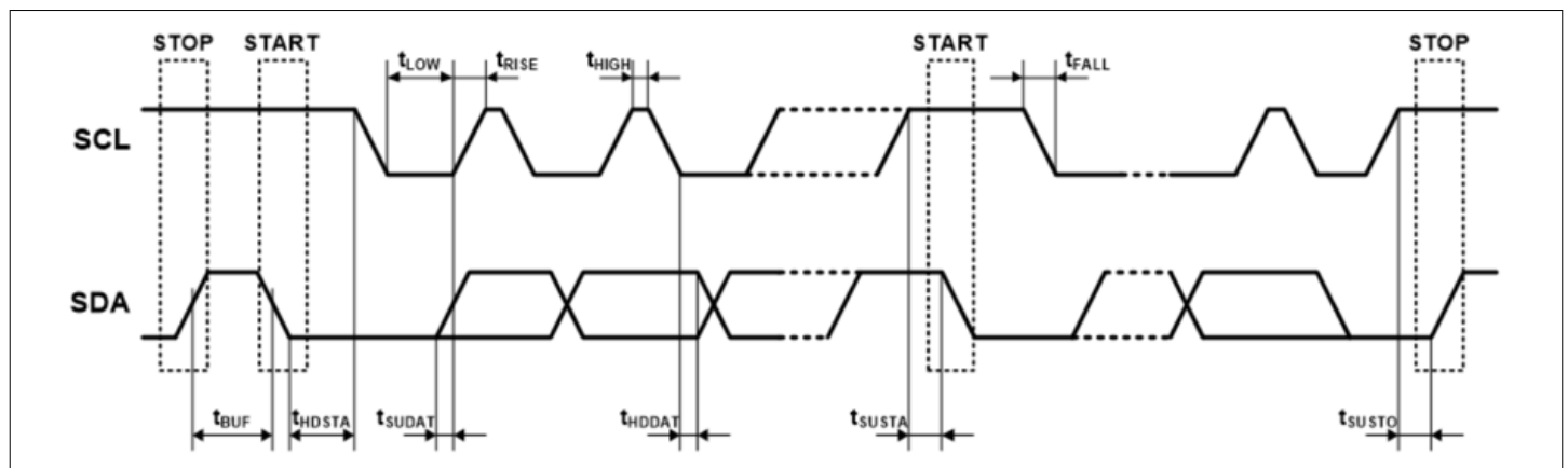
Figure 6 Serial interface timing diagram
