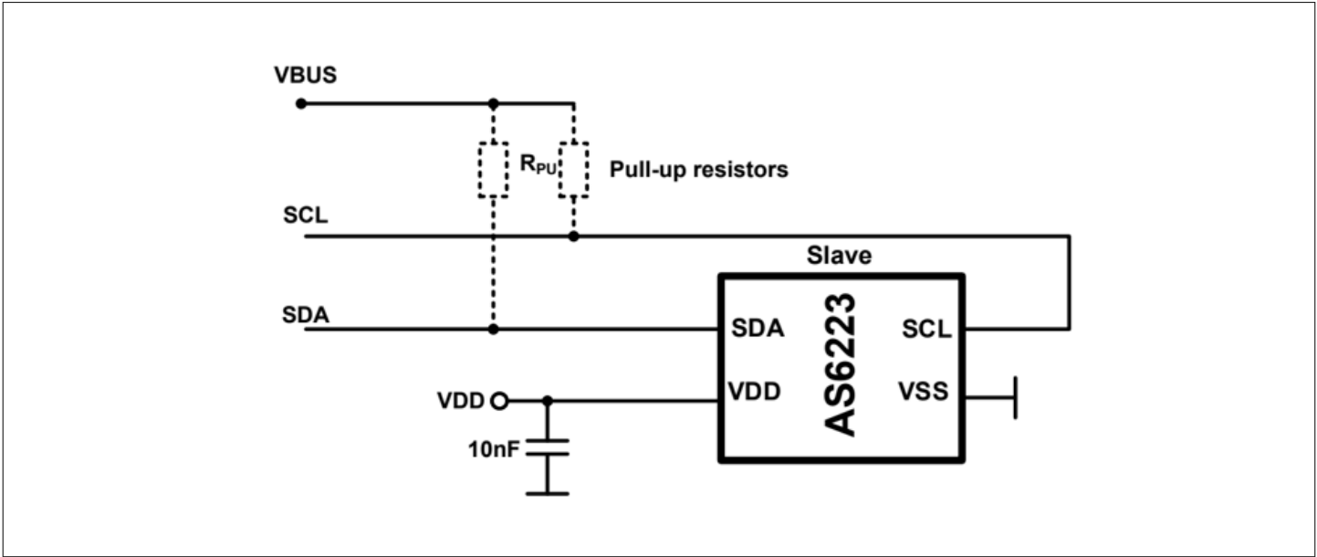
Figure 9 Schematic with external components
