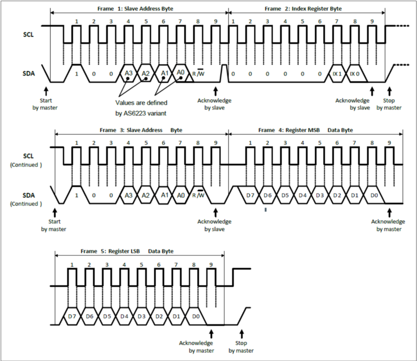
Figure 8 Timing diagram for word read
