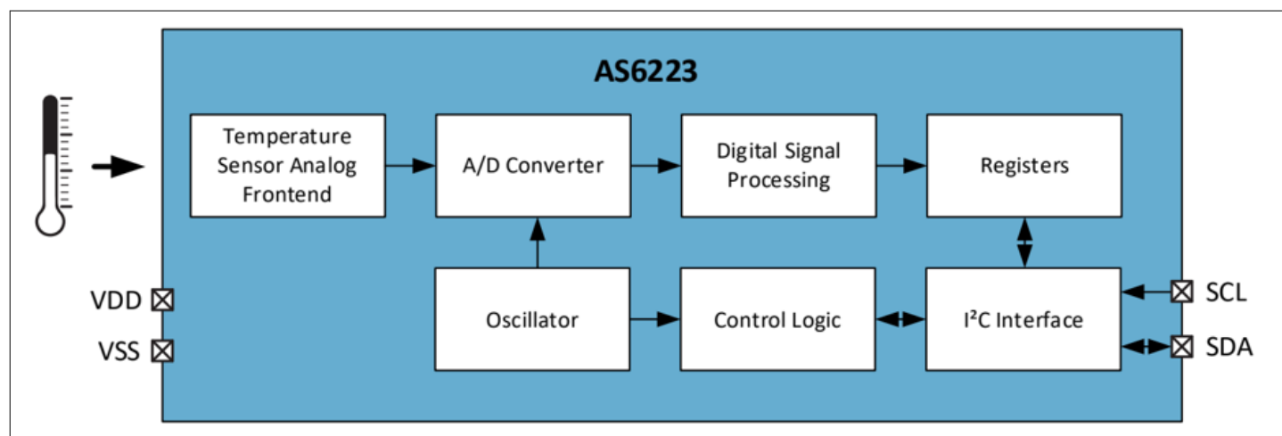
Figure 1 Functional blocks of AS6223
