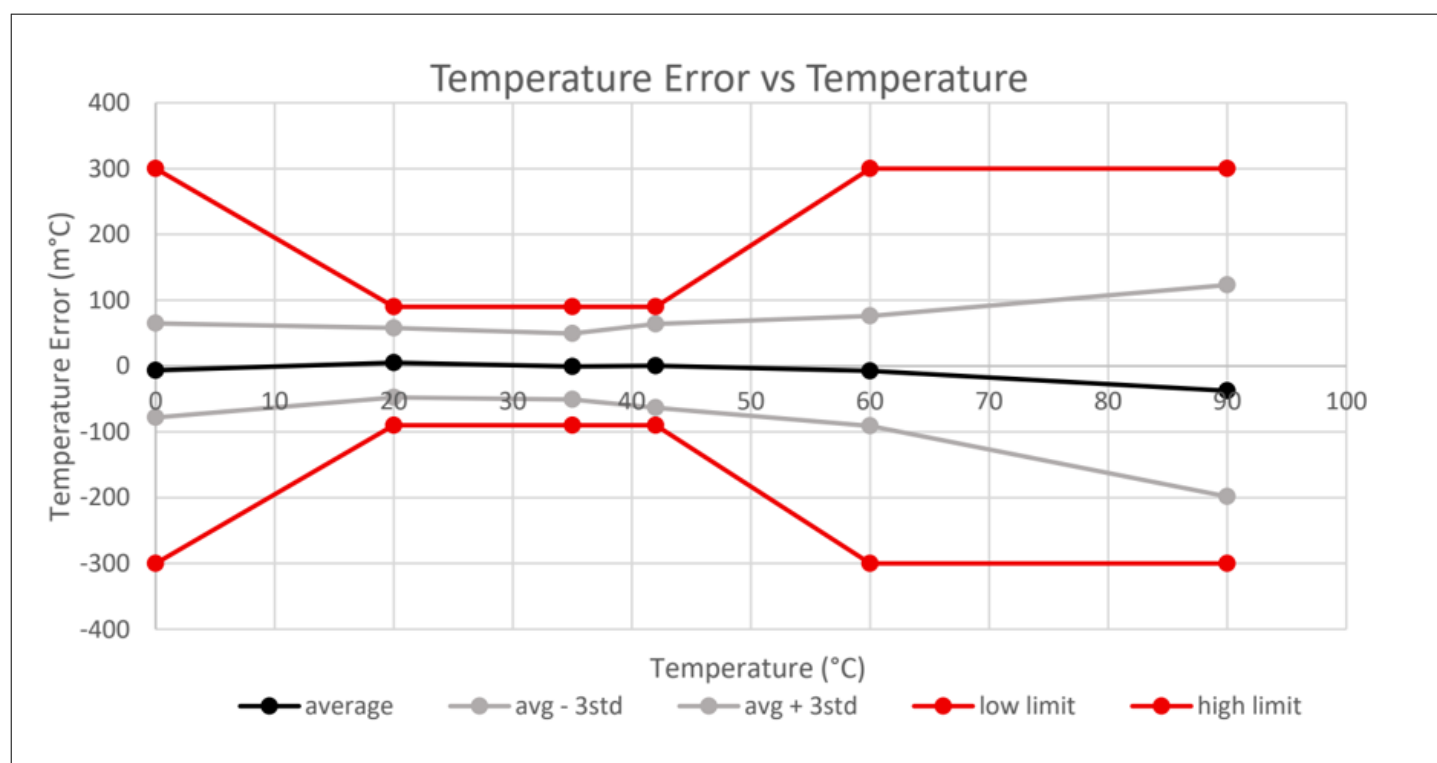
Figure 3 AS6223 measurement accuracy over temperature
