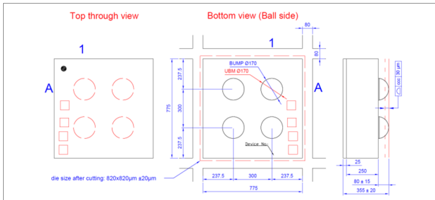
Figure 10 WLCSP outline drawing (Bottom & side view)
