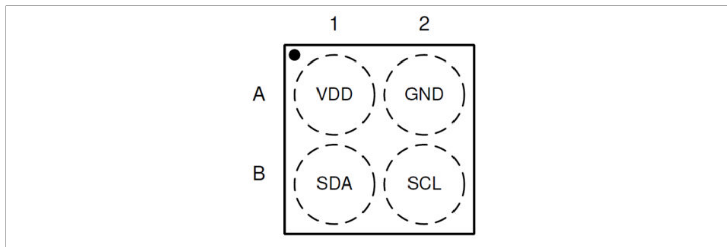
Figure 2 Pin diagram of AS6223 (WLCSP)
