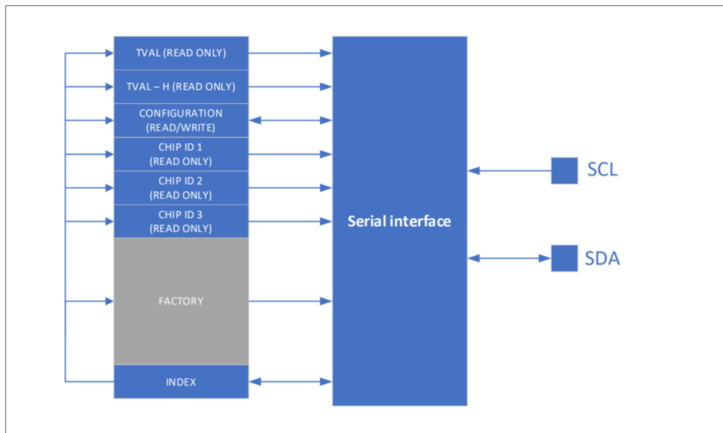
Figure 4 Register map with serial interface
