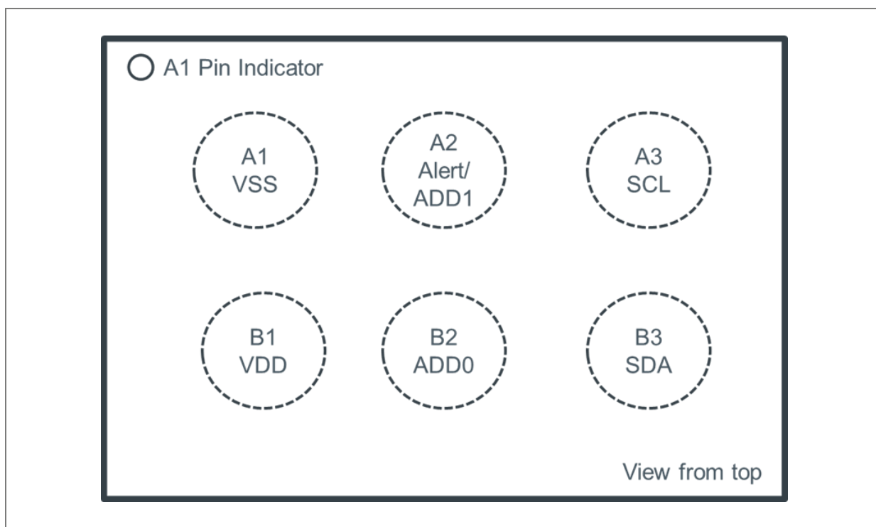
Figure 2: Pin assignment WLCSP
