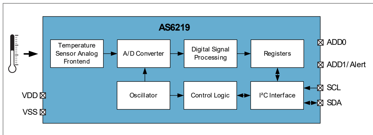
Figure 1: Functional blocks of AS6219
