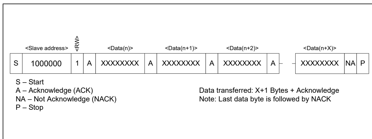
Figure 20: Data Read (Slave Transmitter Mode)
