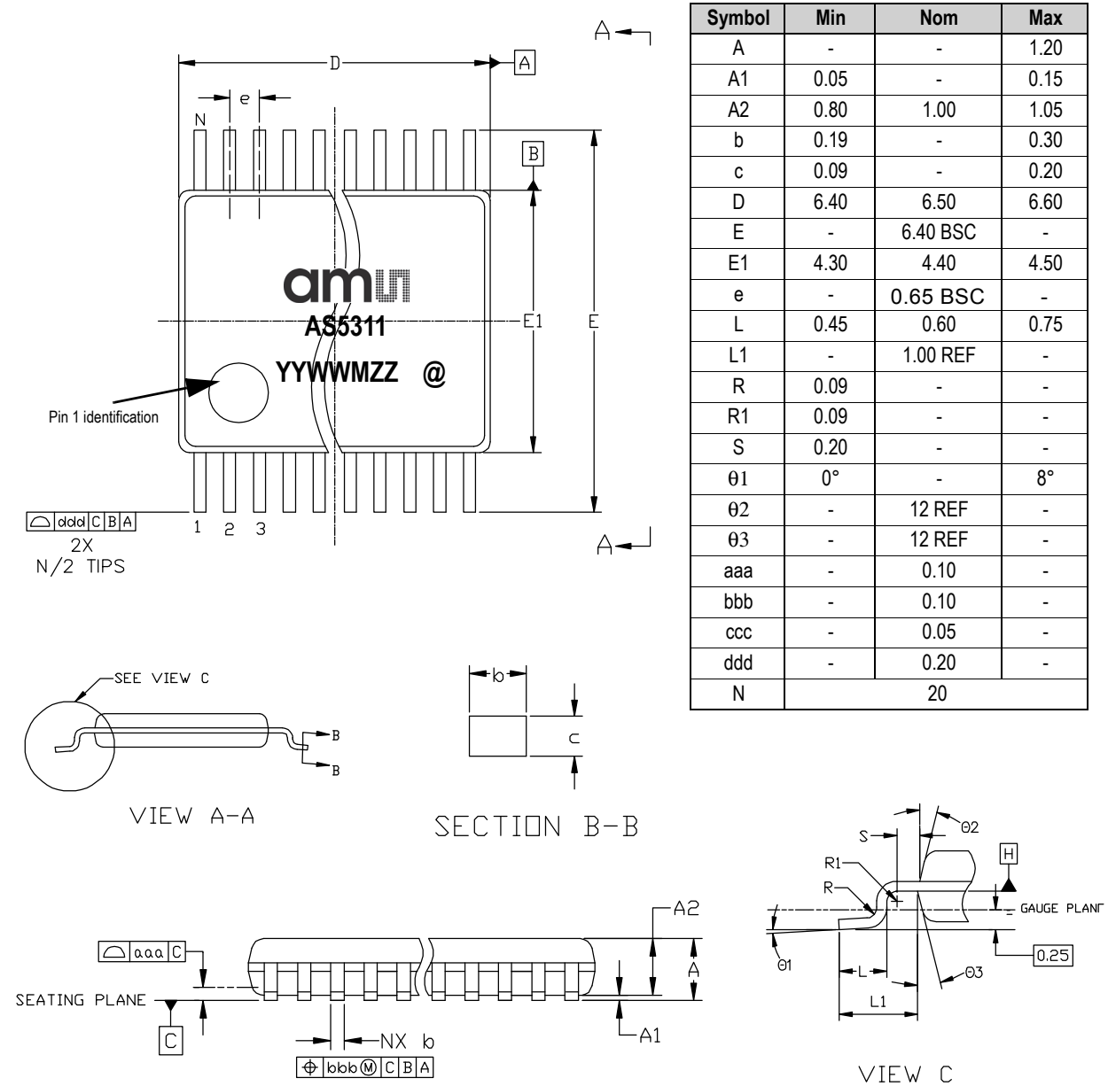
Figure 19. 20-pin TSSOP Package Dimensions and Hall Array Location
