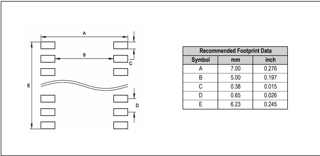
Figure 20. PCB Footprint
