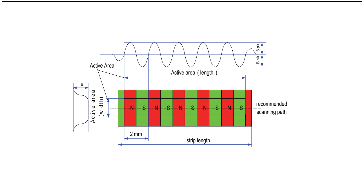
Figure 13. Active Area of Strip Magnet
