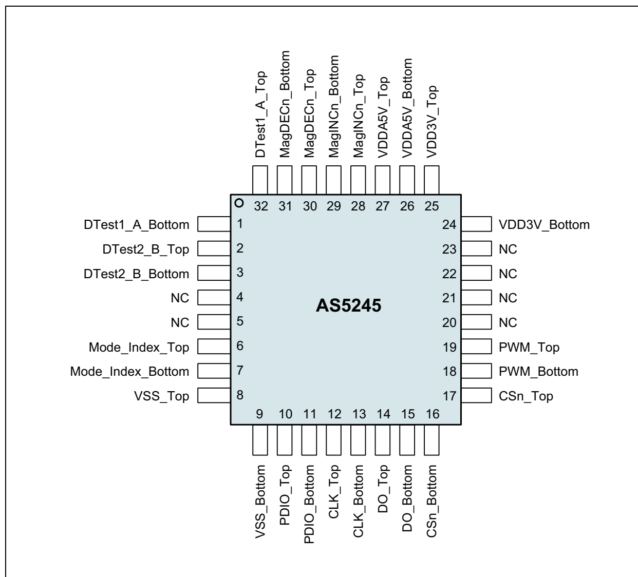
Figure 3: Pin Assignments (Top View)
