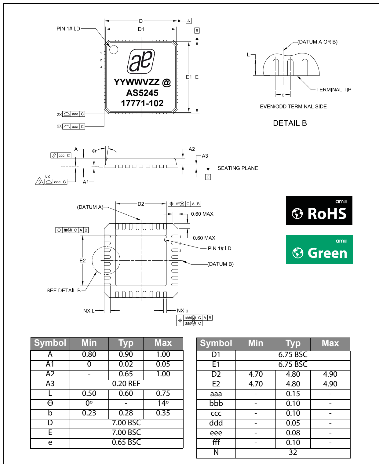
Figure 34: Package Drawing
