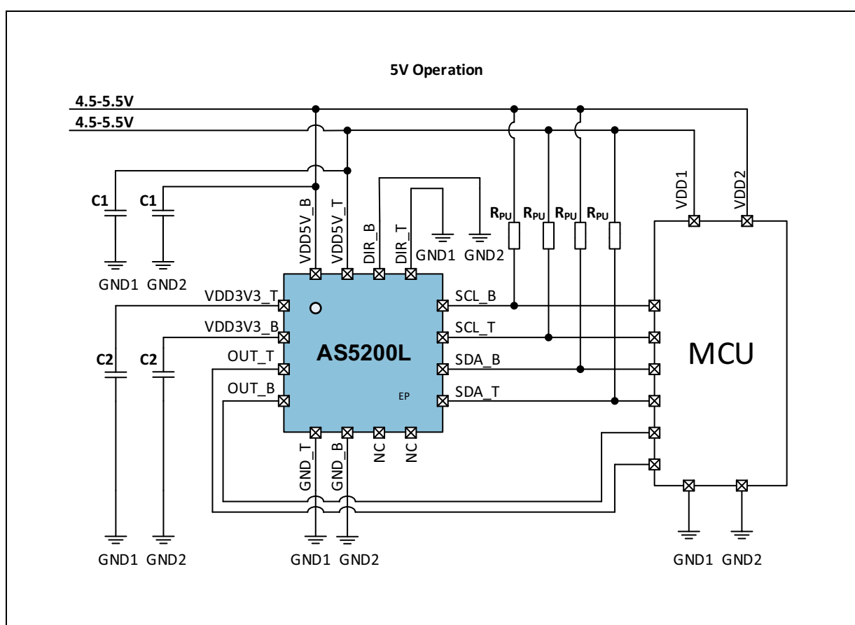
Figure 13: Application diagram for angle readout and programming with I 2 C
