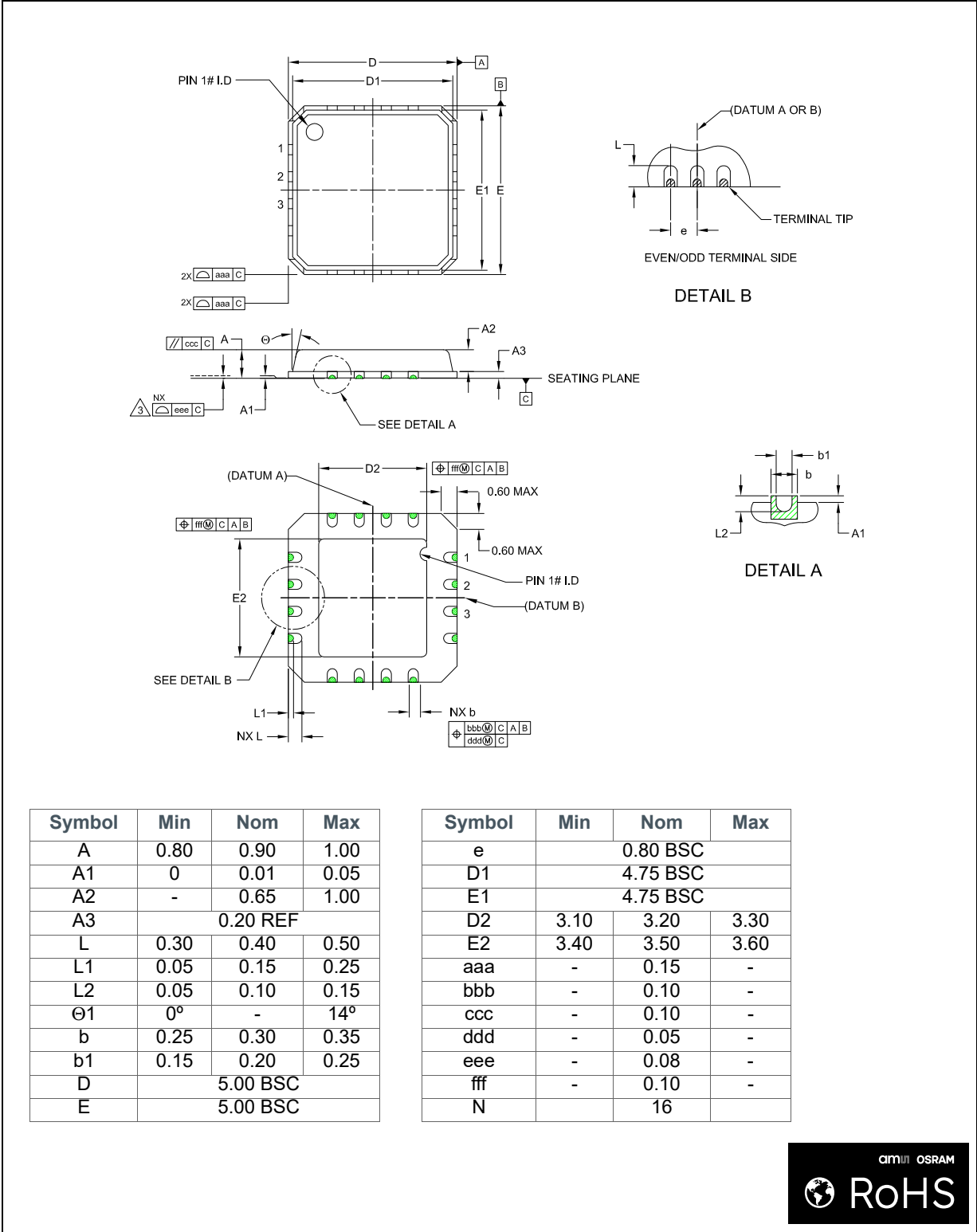
Figure 16: MLF-16 package outline drawing
