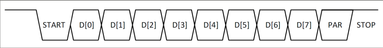
Figure 9: UART protocol frame
