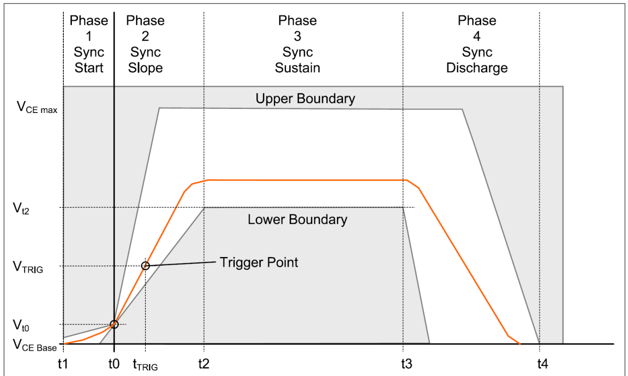
Figure 4: Synchronization signal
