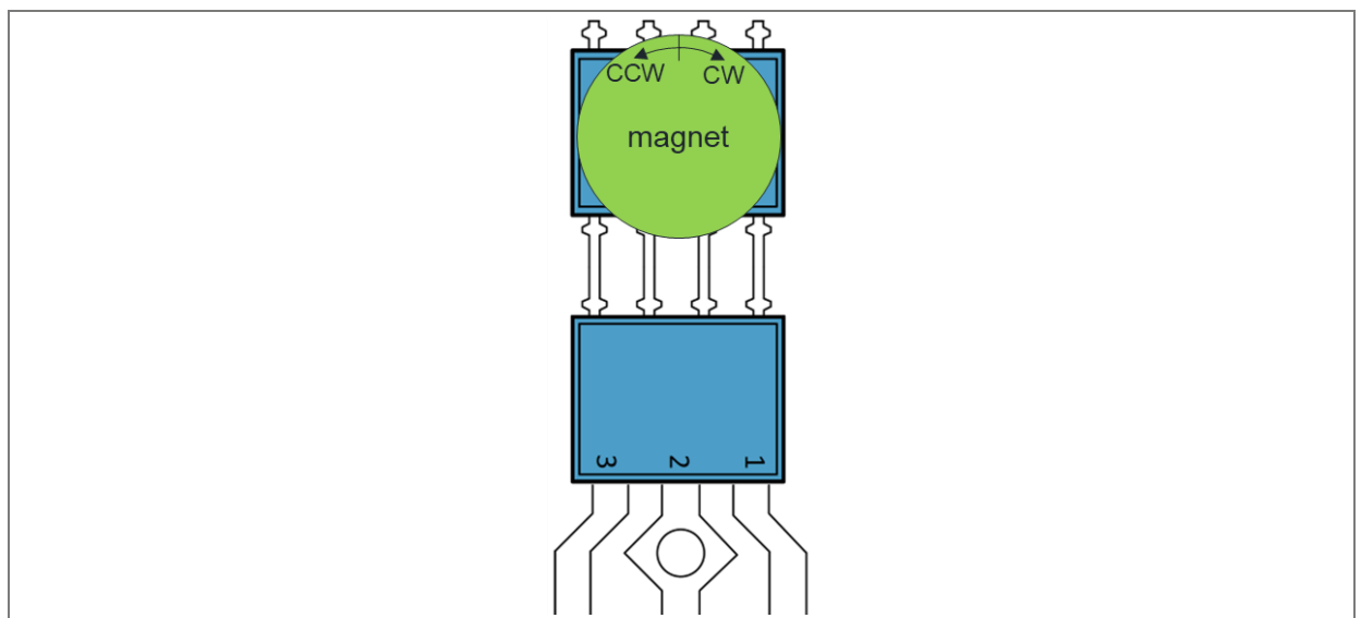
Figure 19: Definition of clockwise (CW) and counterclockwise (CCW) rotation direction
