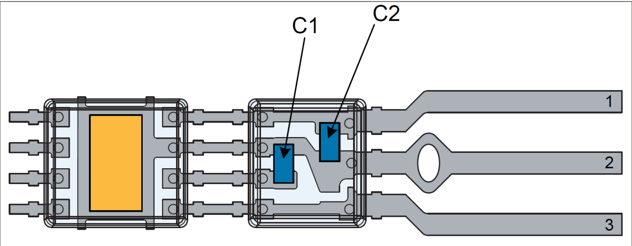
Figure 35: AS5173 components
