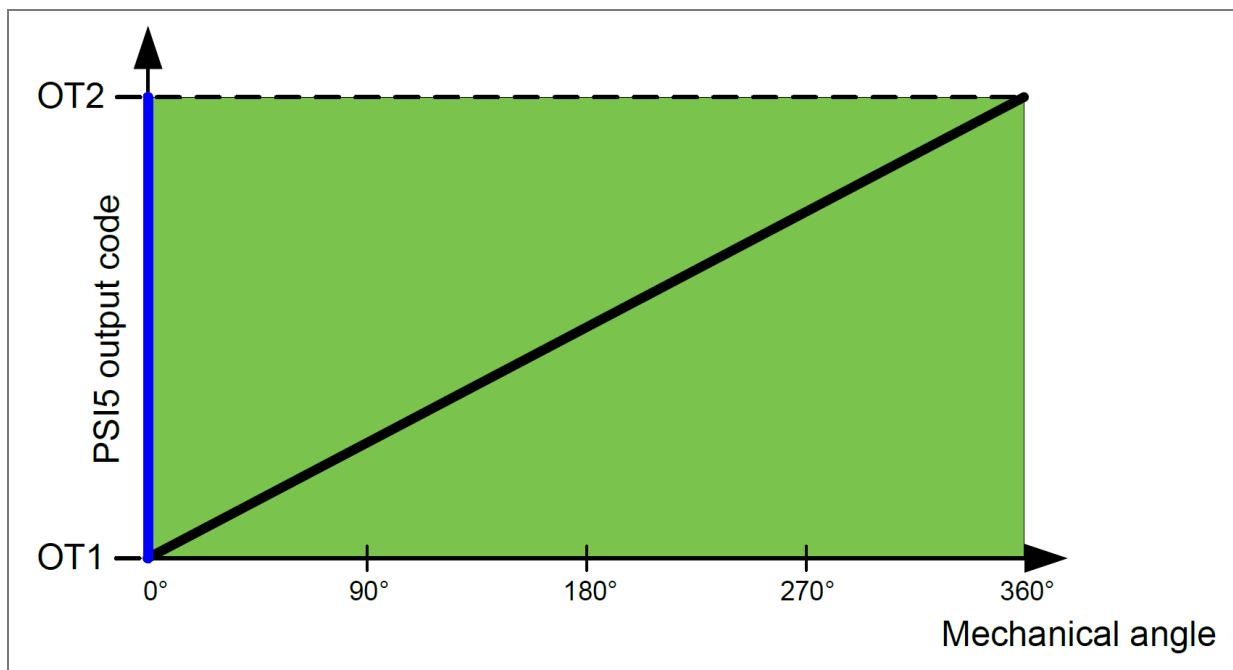
Figure 13: Single quadrant
