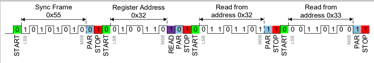
Figure 11: Example of READ (Reg[0x32] = 0xB6 and Reg [0x33] = 0x2C)
