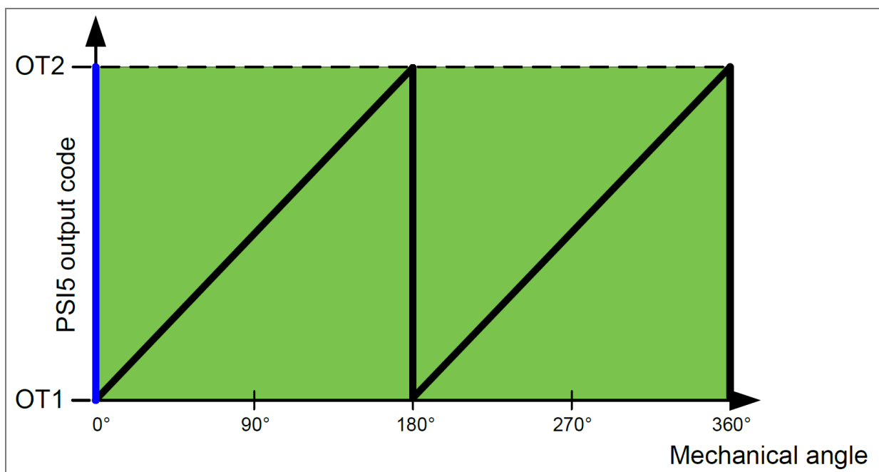
Figure 14: Dual quadrant
