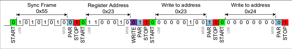
Figure 10: Example of WRITE (Reg[0x23] = 0x20 and Reg [0x24] = 0x00)
