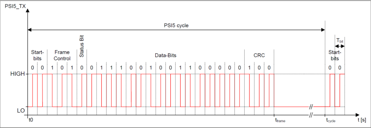
Figure 28: Asynchronous modes A20CRC-200/1H and A20CRC-300/1L
