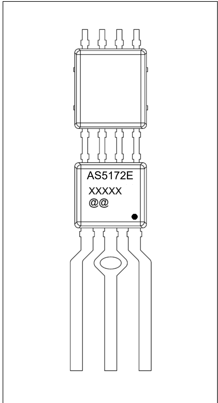
Figure 76: SIP Marking Drawing AS5172E
