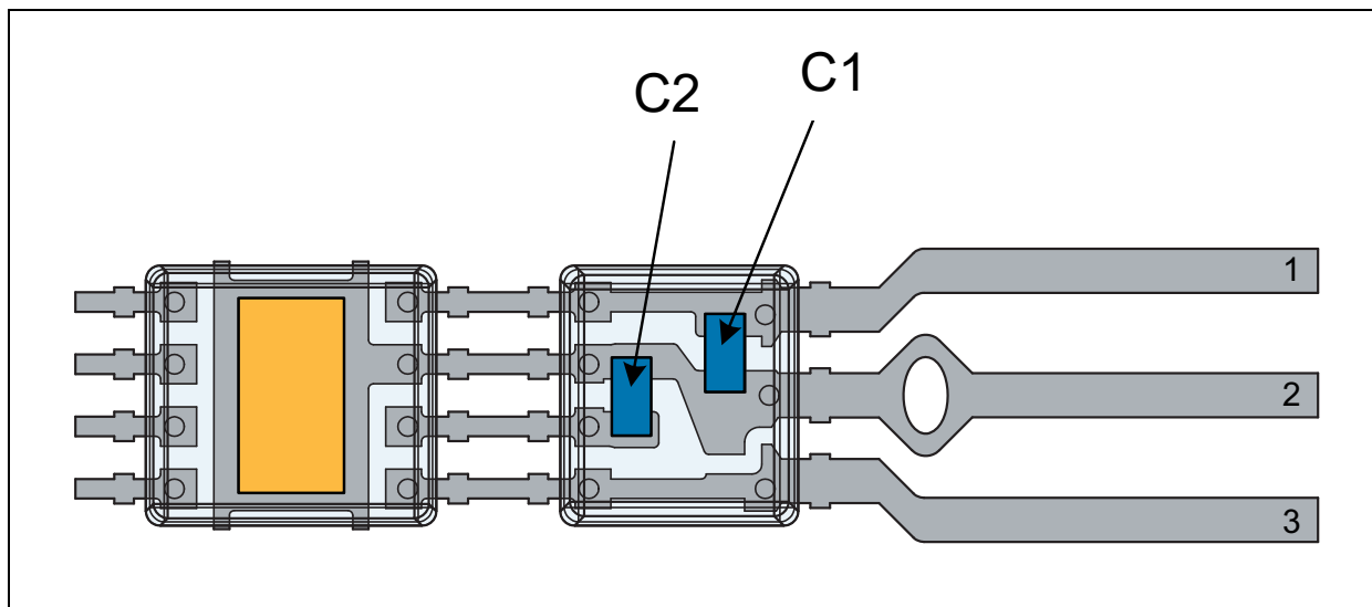
Figure 73: AS5172E/F Components
