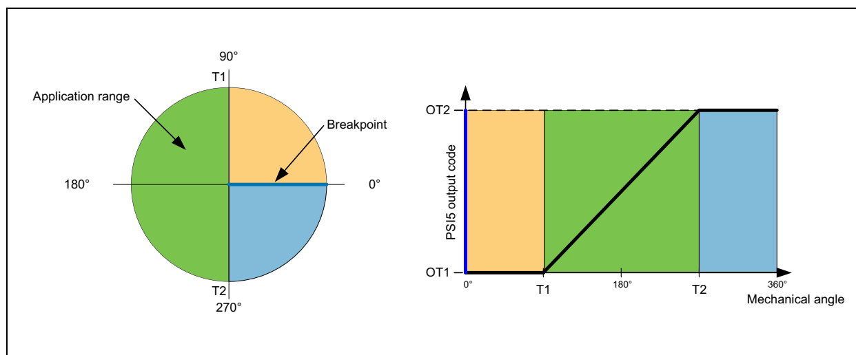
Figure 27: Transfer Function
