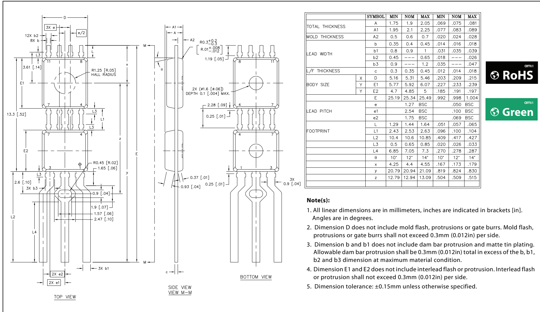
Figure 75: SIP Package Outline Drawing
