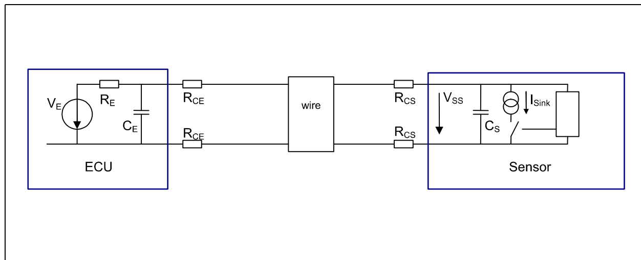
Figure 69: Asynchronous Single Sensor Configuration
