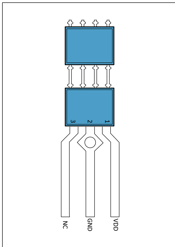
Figure 3: AS5172E/F in SIP Package
