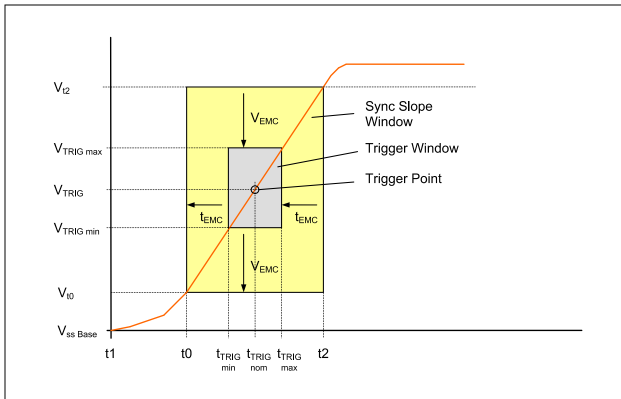
Figure 13: Trigger Window
