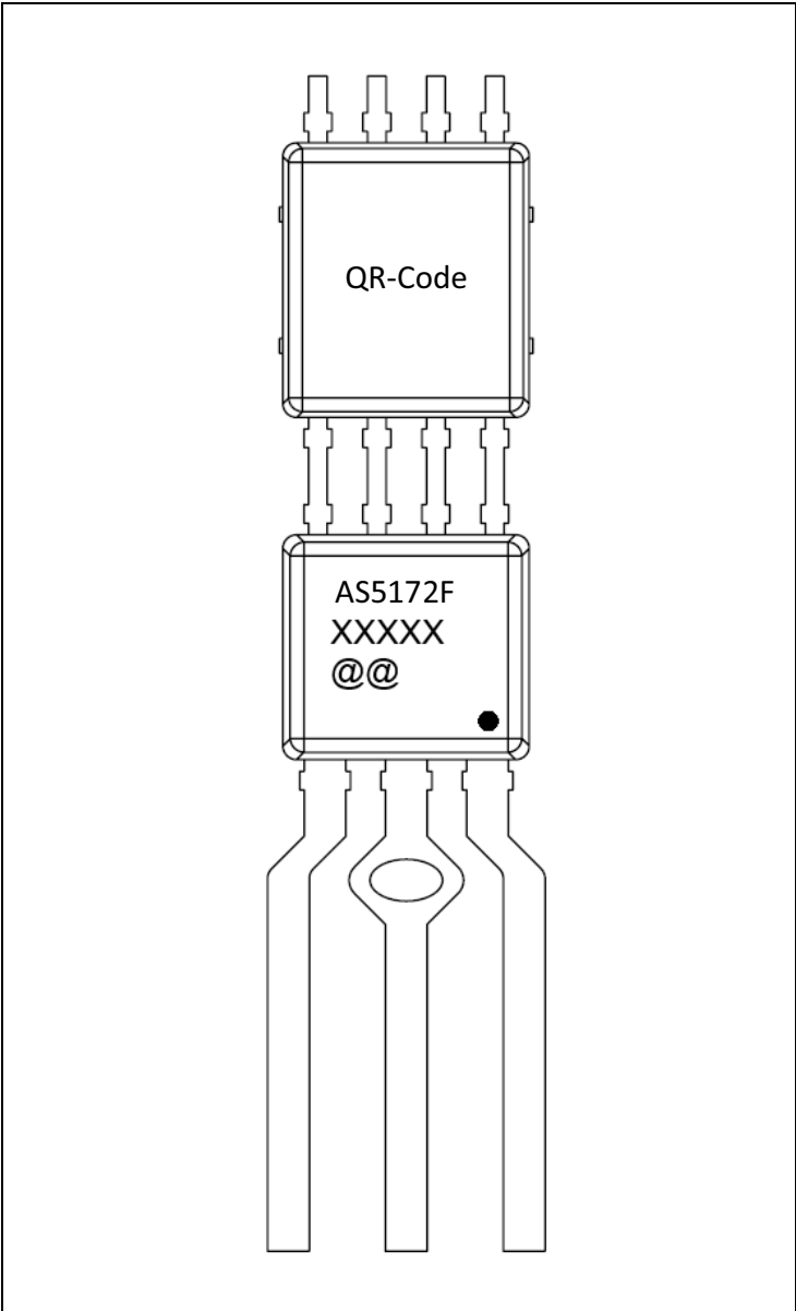
Figure 78: SIP Package Code
