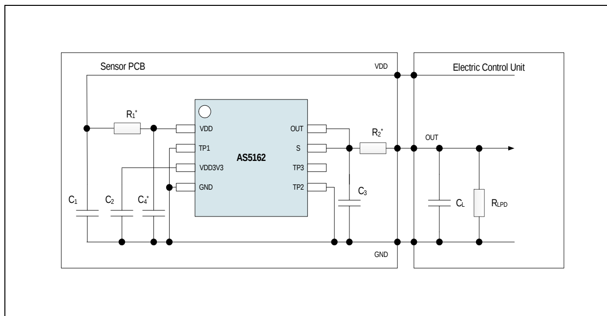
Figure 23: Recommended Schematic of Pull-Down Configuration
