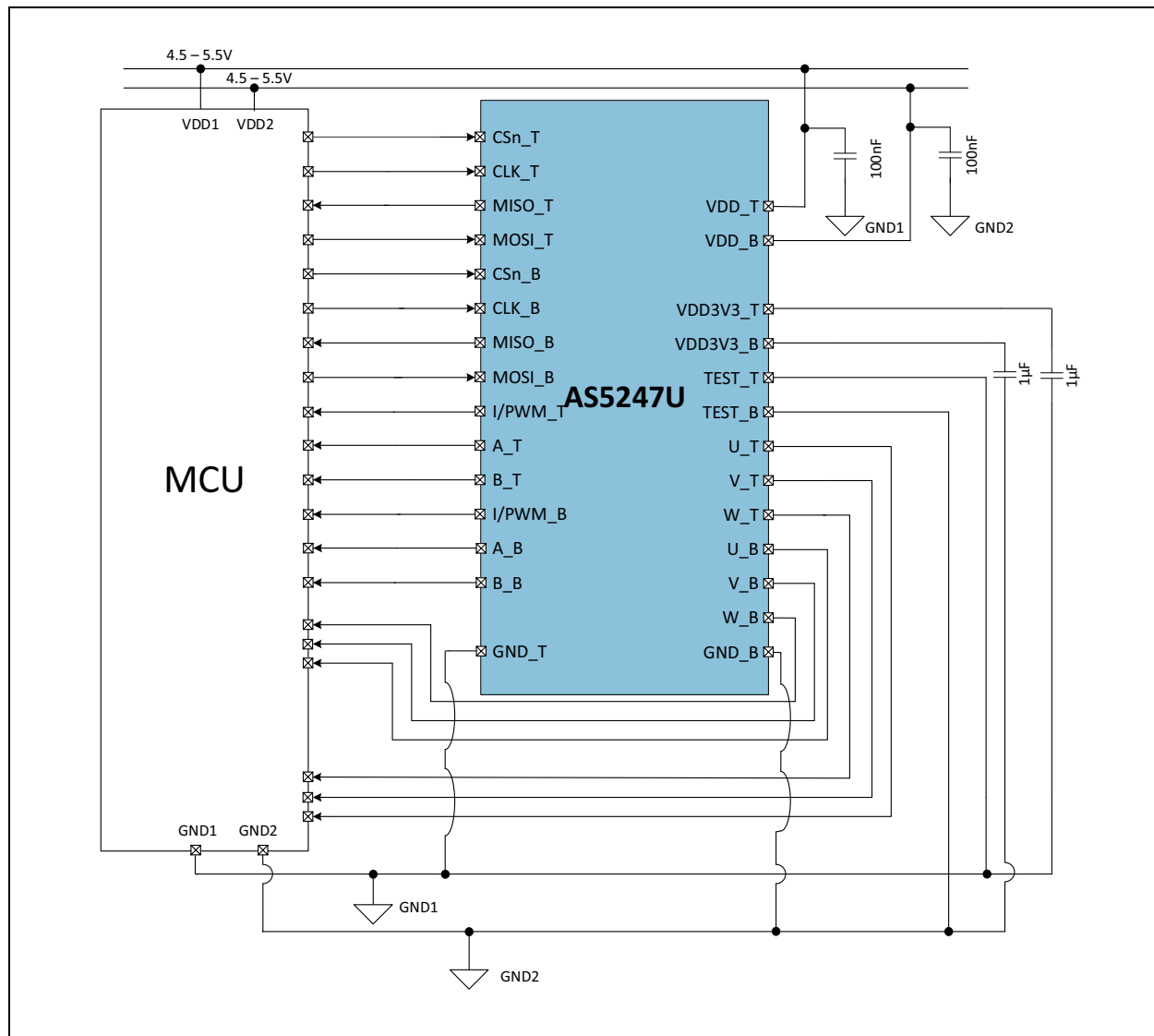
Figure 67: Minimum Circuit Diagram for the AS5247U
