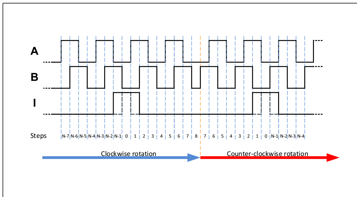
Figure 52: ABI Signals
