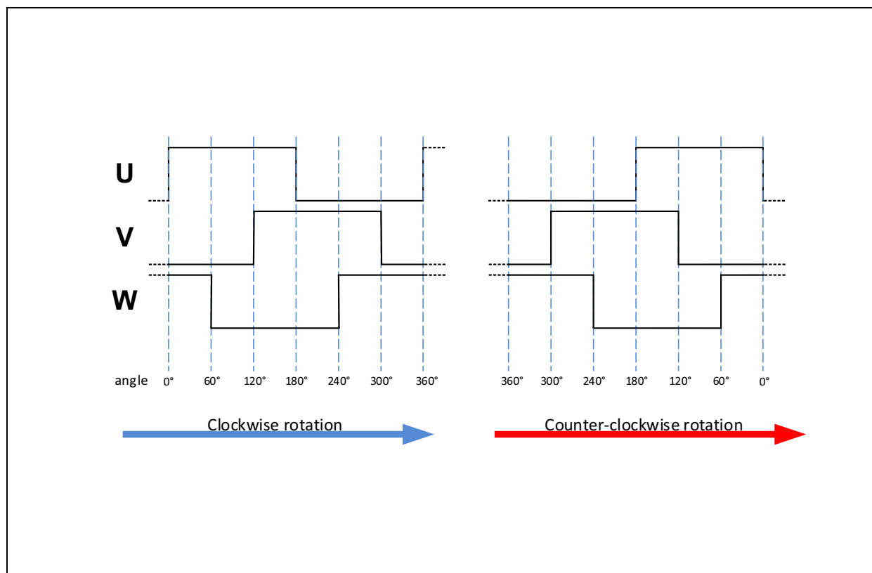
Figure 54: UVW Signals
