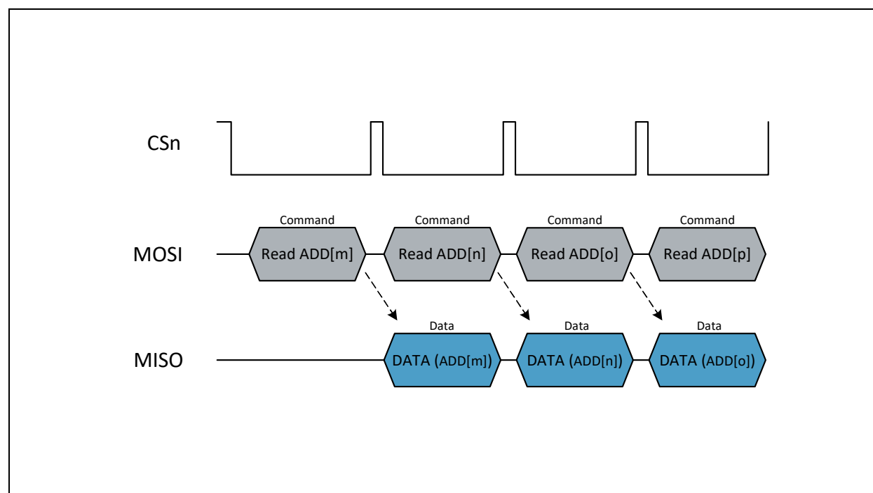
Figure 31: SPI Read
