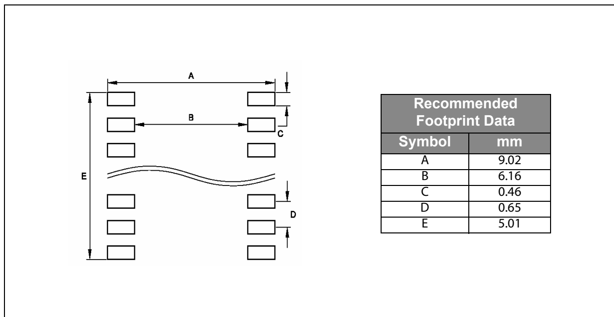
Figure 41: PCB Footprint
