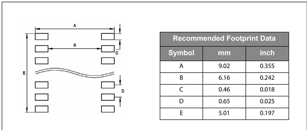
Figure 49: PCB Footprint
