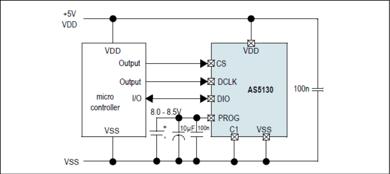
Figure 24: External Circuitry for OTP Programming
