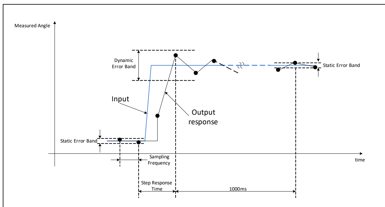
Figure 26: Step Response
