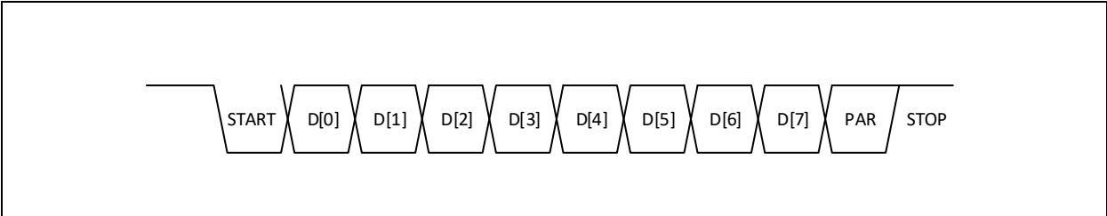
Figure 19: UART Frame
