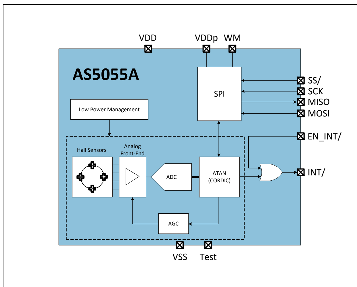
Figure 2: AS5055A Block Diagram
