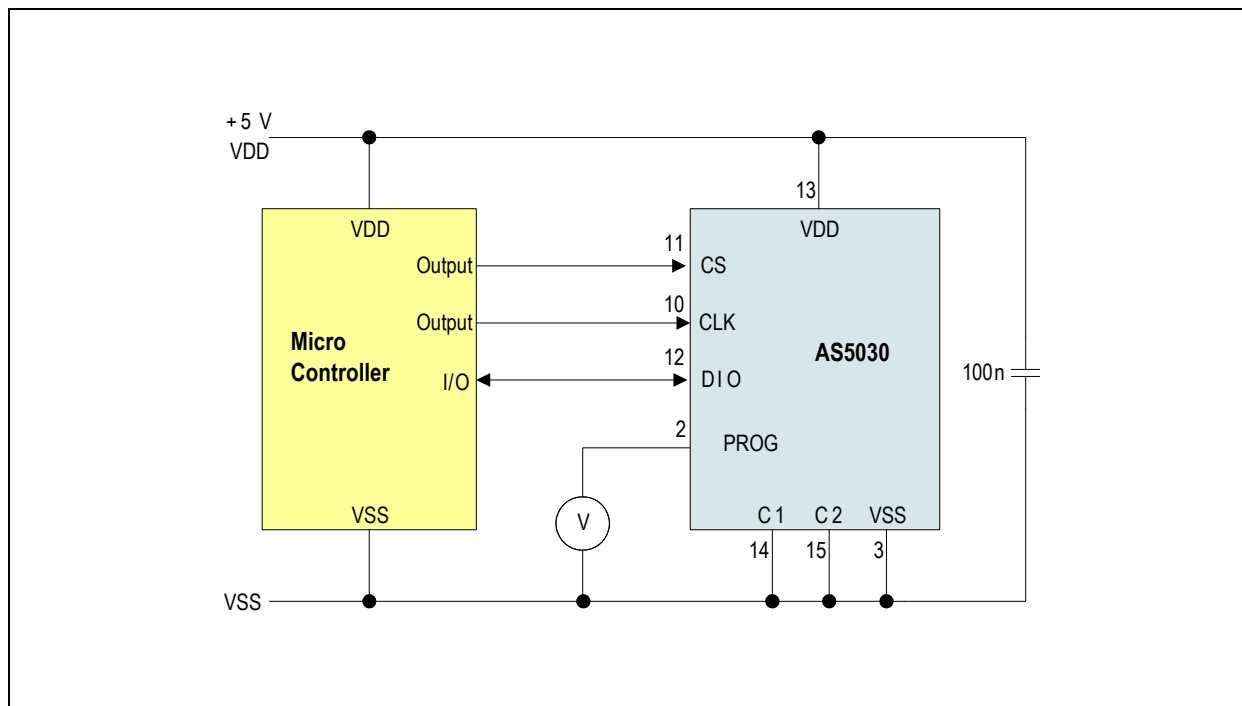
Figure 49: Analog OTP Verification
