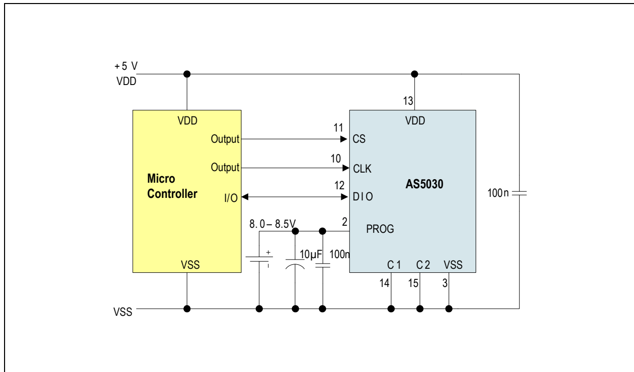
Figure 48: OTP Programming Connection
