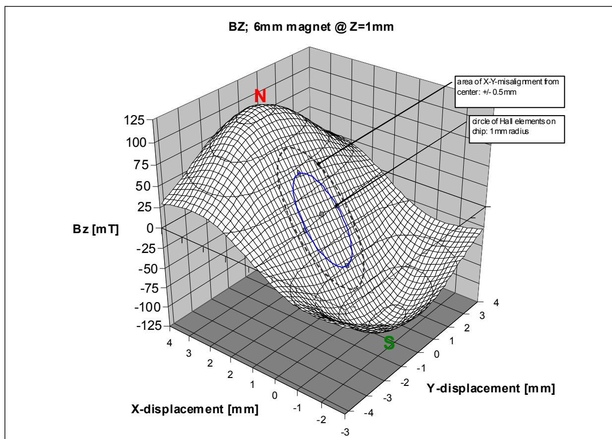
Figure 62: Vertical Magnetic Field Distribution of a Cylindrical 6mm \varnothing Diametric Magnetized Magnet at 1mm Gap
