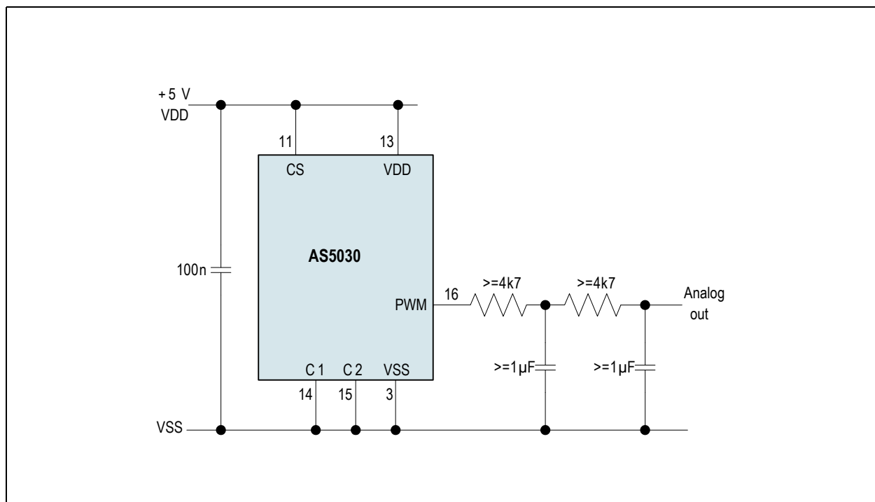
Figure 35: Data Transmission with Pulse Width Modulated (PWM) Output
