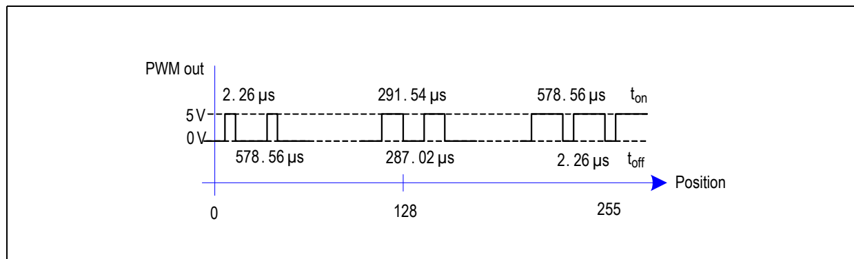
Figure 33: PWM Timing
