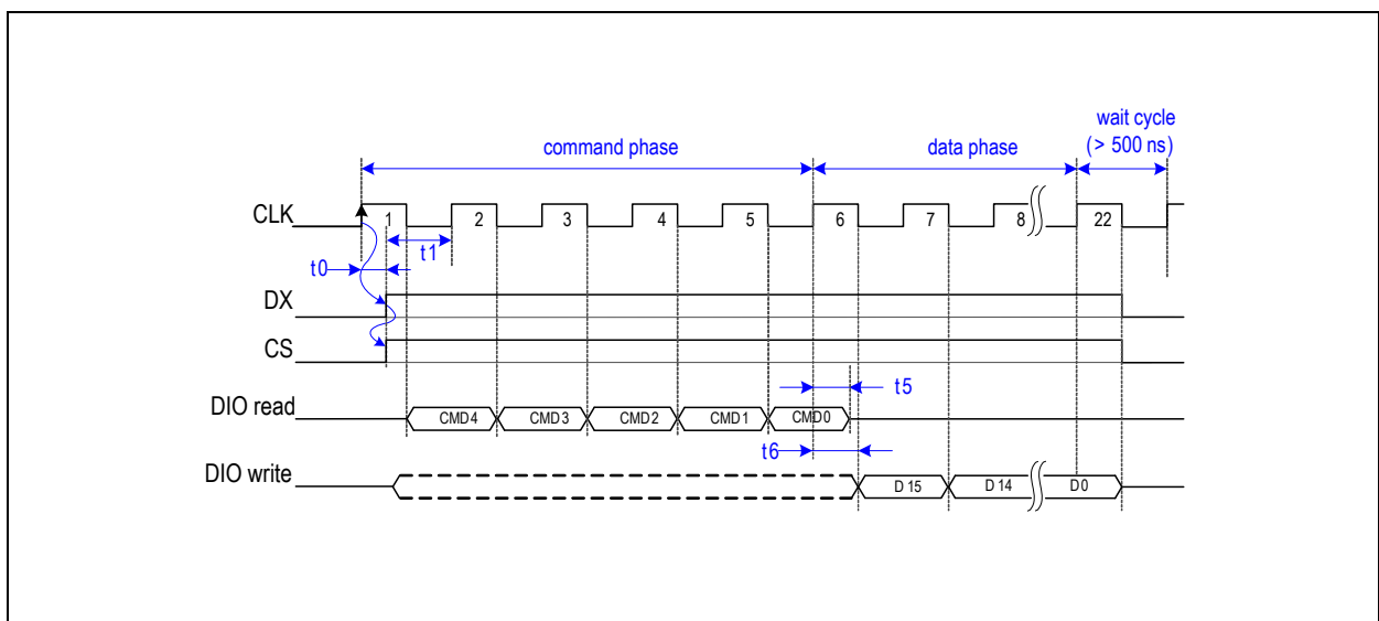
Figure 27: Timing Diagram in 2-Wire SSI Mode
