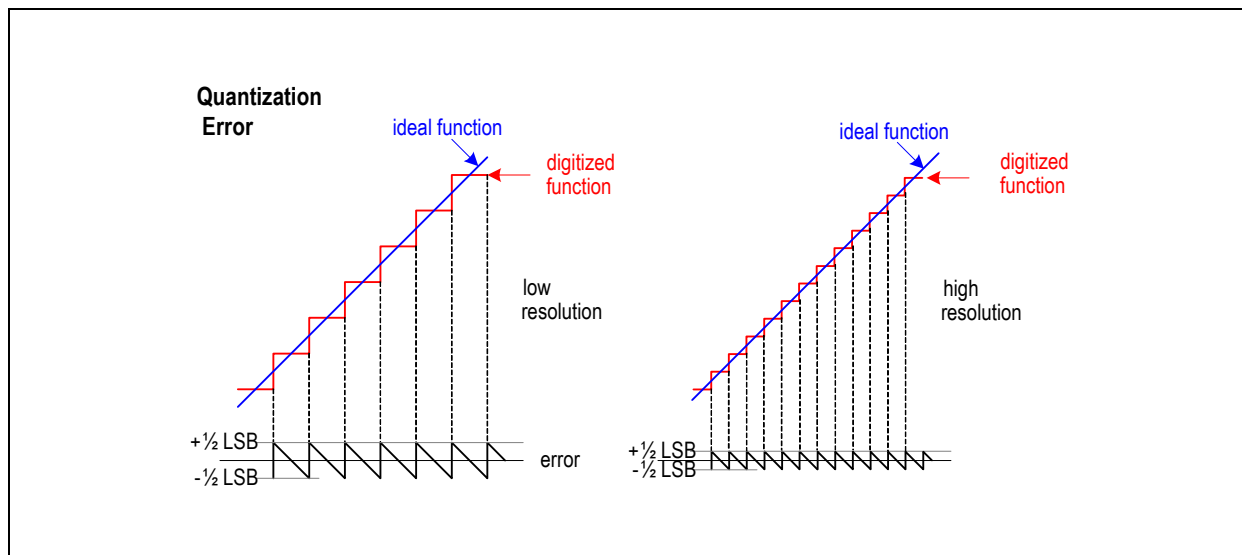
Figure 57: Quantization Error of a Low Resolution and a High Resolution System
