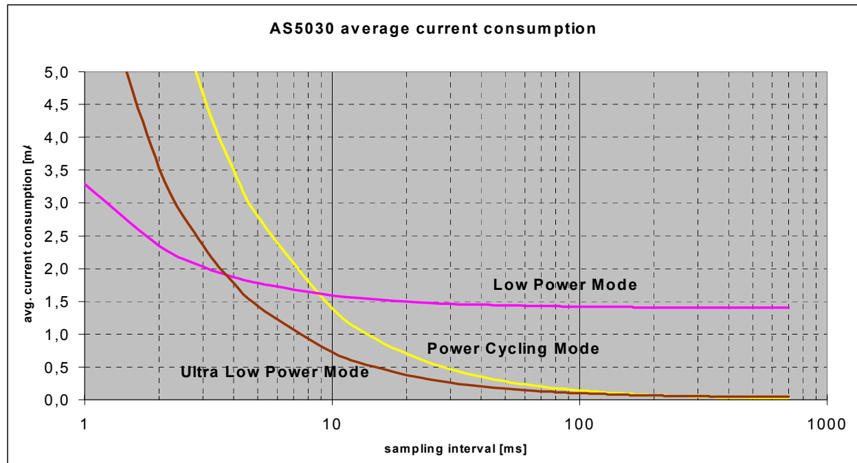
Figure 56: Average Current Consumption of Reduced Power Modes
