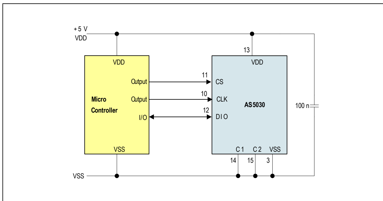
Figure 20: SSI Read/Write Serial Data Transmission
