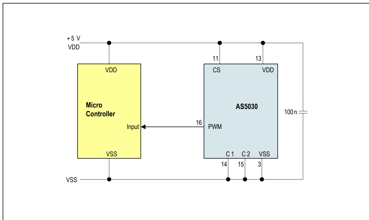
Figure 32: Data Transmission with Pulse Width Modulated (PWM) Output
