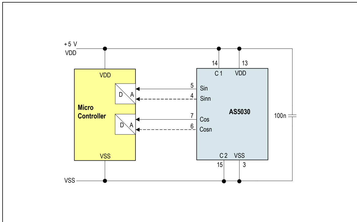
Figure 37: Sine and Cosine Outputs for External Angle Calculation
