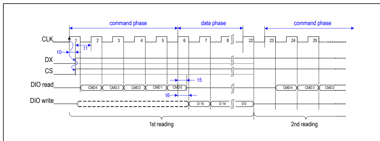
Figure 28: Timing Diagram in 2-Wire SSI Continuous Readout
