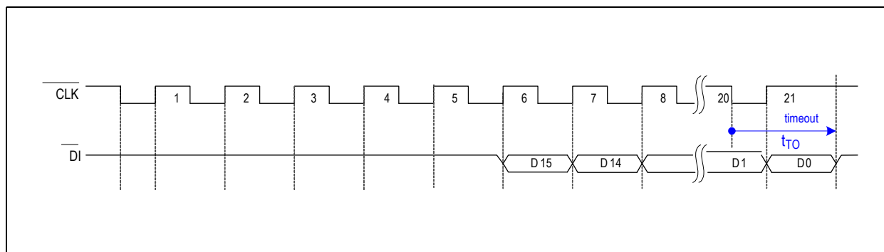
Figure 30: Timing Diagram in 2-Wire Read-Only Mode (differential transmission)
