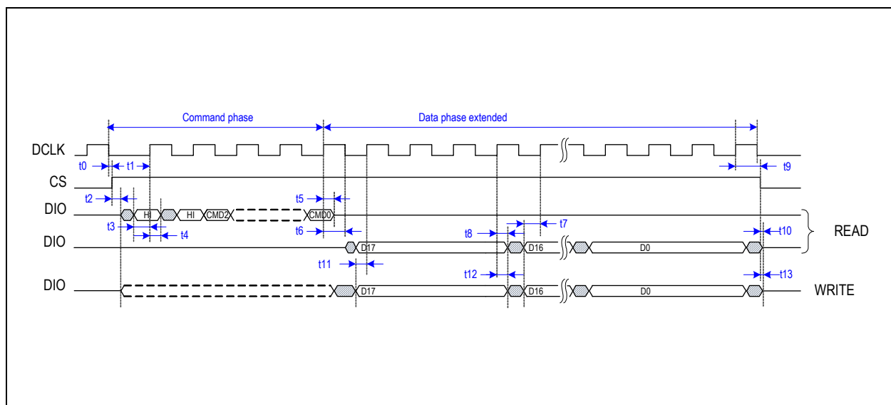
Figure 47: Timing Diagram in OTP 18-Bit Read/Write Mode
