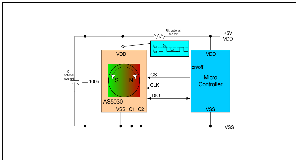
Figure 52: Low Power Mode and Ultra-Low Power Mode Connection
