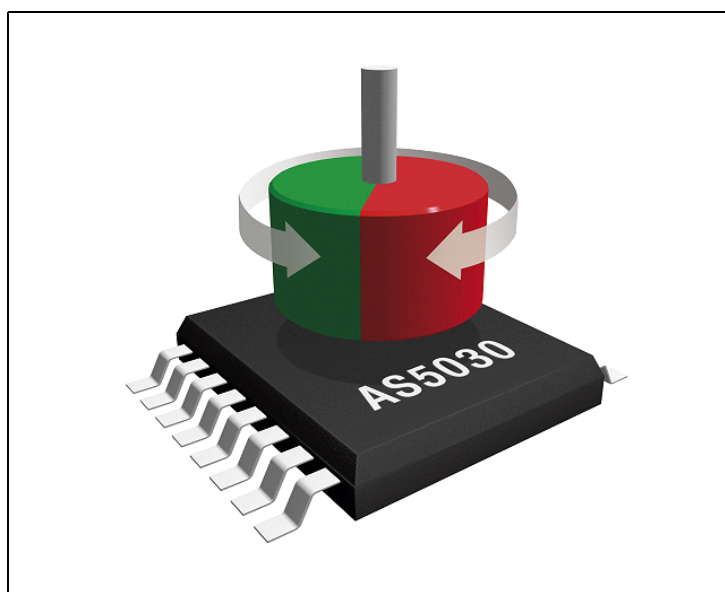
Figure 2: Typical Arrangement of AS5030 and Magnet
