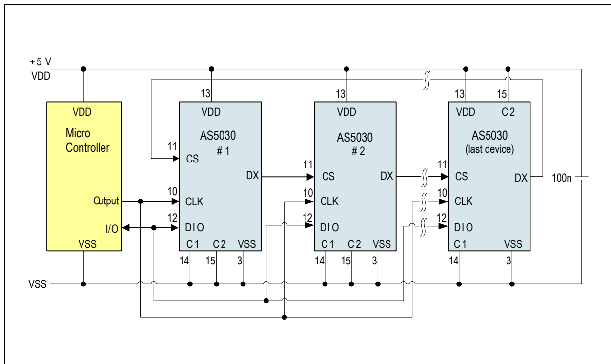
Figure 40: 2-Wire Daisy Chain Mode
