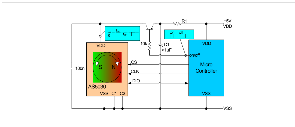
Figure 55: Application Example III: Ultra-low Power Encoder
