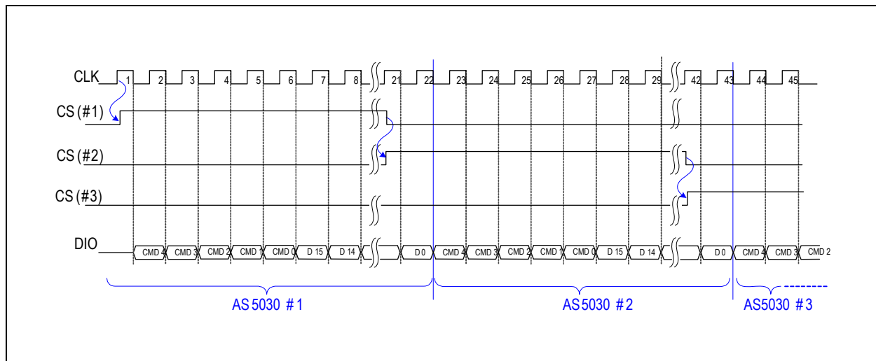
Figure 41: Timing Diagram in 2-Wire Daisy Chain Mode
