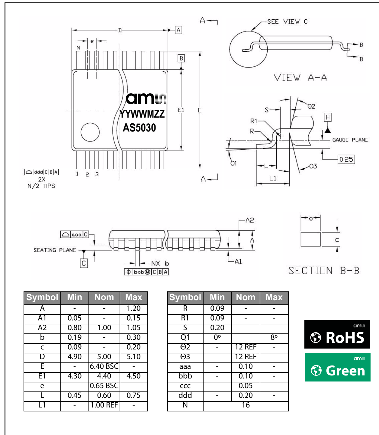
Figure 66: 16-Pin TSSOP Package
