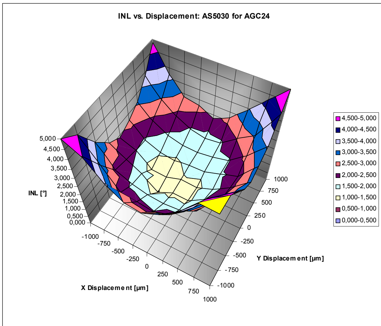
Figure 63: Typical Error Curve of INL Error Over Lateral Displacement (including quantization error)
