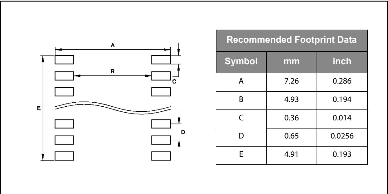
Figure 68: PCB Footprint
