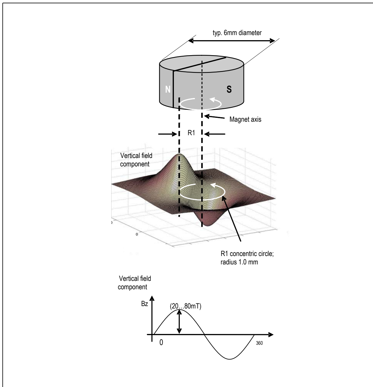
Figure 60: Vertical Magnetic Fields of a Rotating Magnet
