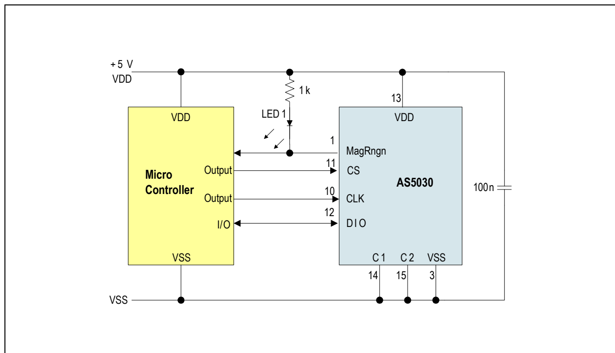
Figure 50: Magnetic Field Strength Indicator
