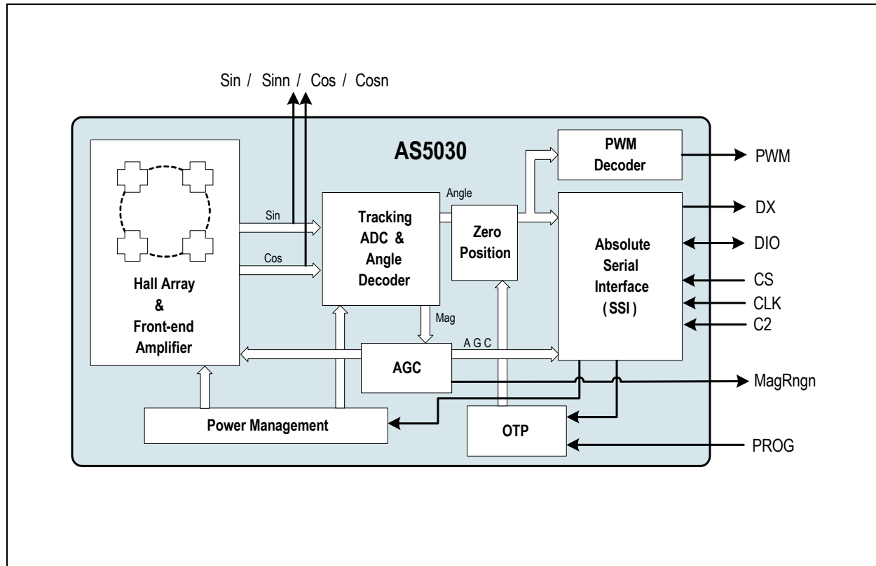
Figure 3: AS5030 Block Diagram
