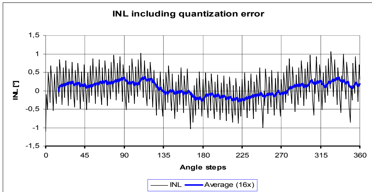
Figure 58: Typical INL Error Over 360°
