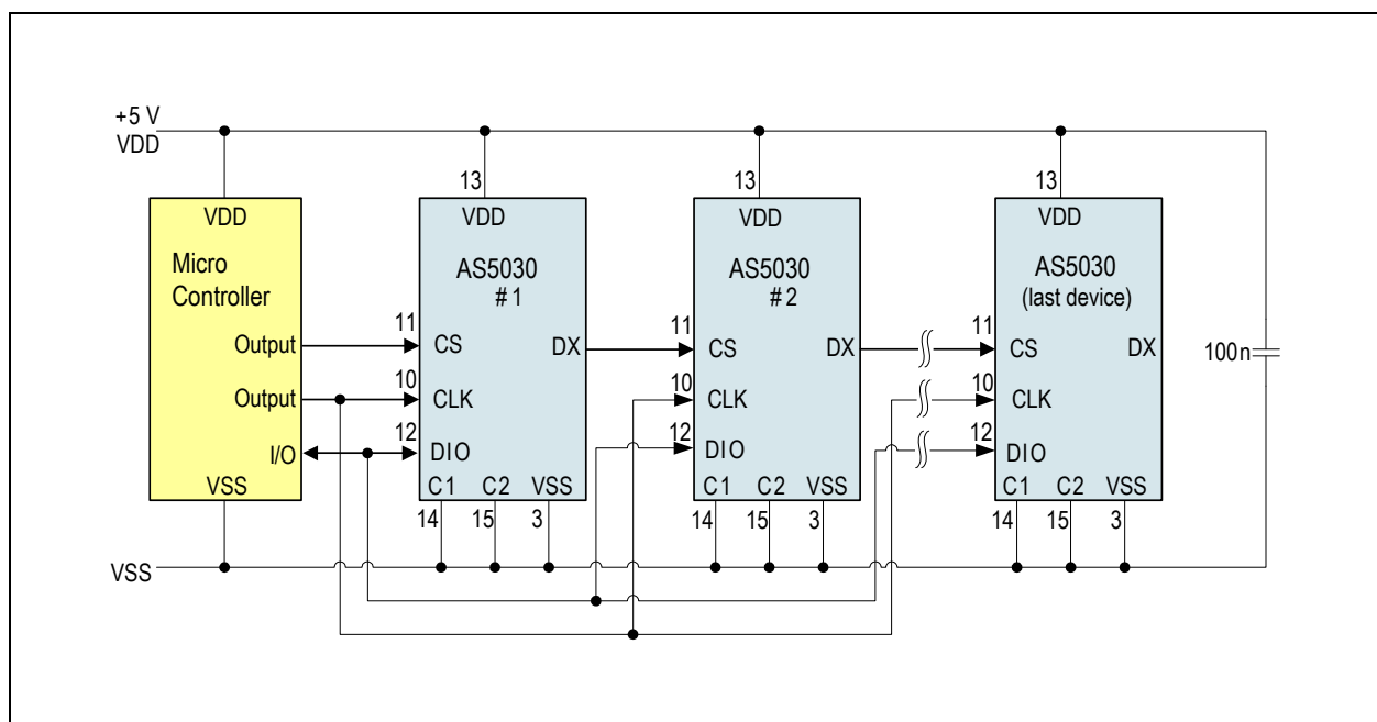
Figure 38: Connection of Devices in 3-Wire Daisy Chain Mode
