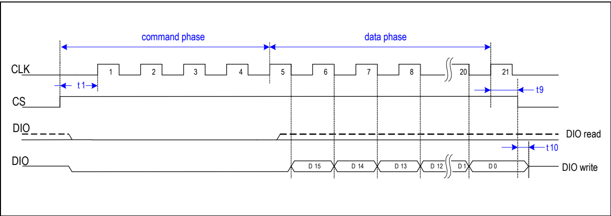
Figure 24: Timing Diagram in 2-Wire and 3-Wire SSI Mode
