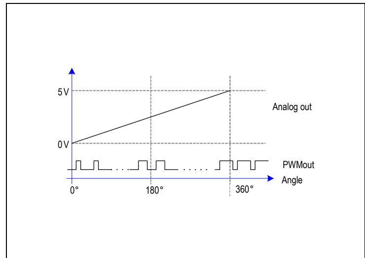
Figure 36: Relation of PWM/Analog Output with Angle
