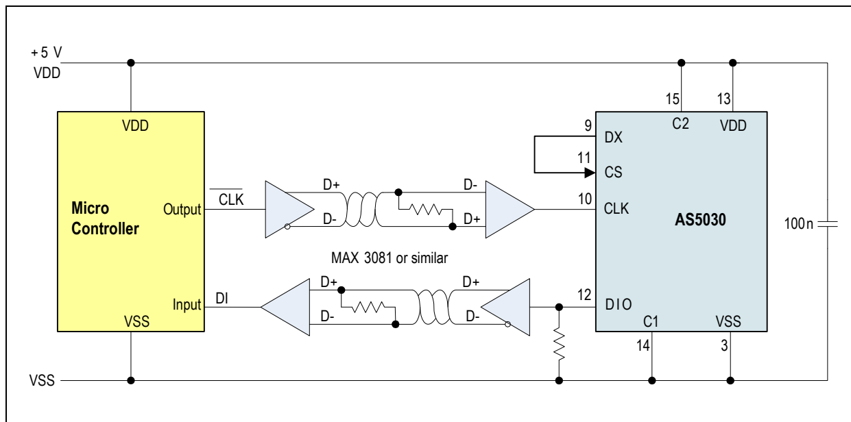
Figure 29: 2-Wire SSI Read-Only Mode
