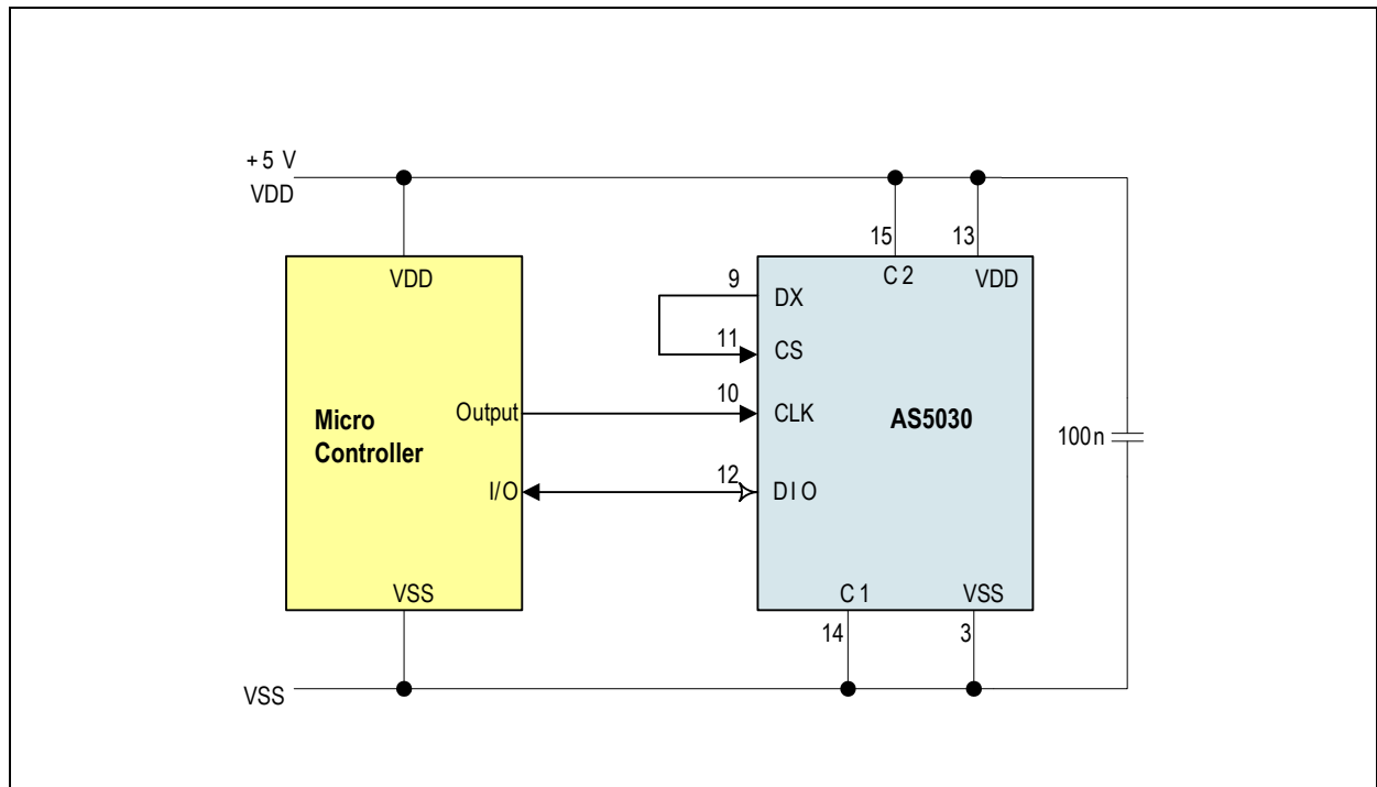
Figure 26: SSI R/W Mode 2-Wire Data Transmission
