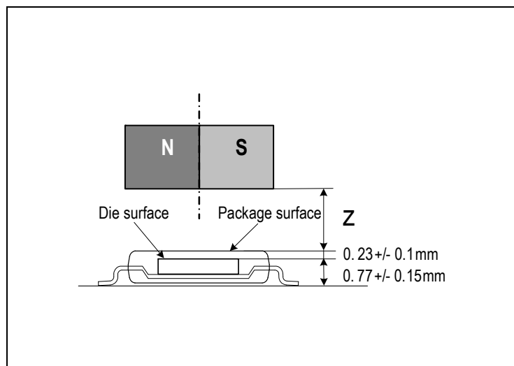
Figure 65: Vertical Placement of the Magnet
