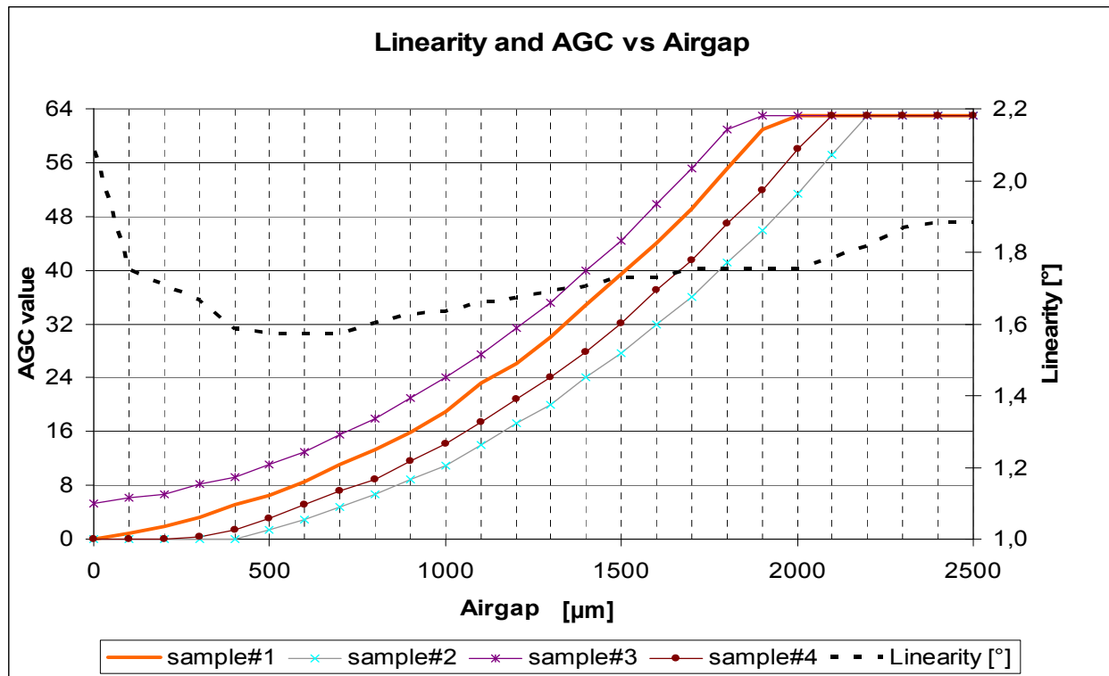
Figure 59: Typical Curves for Vertical Distance Versus ACG Value on Several Untrimmed Samples
