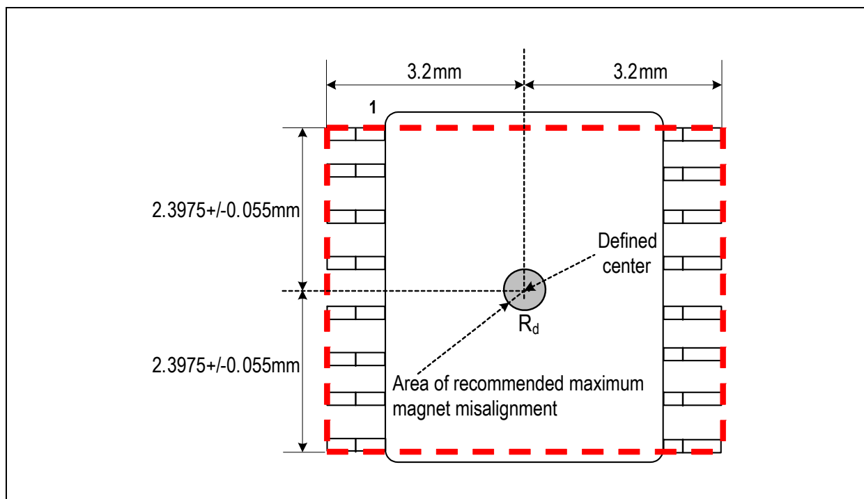
Figure 64: Defined Chip Center and Magnet Displacement Radius
