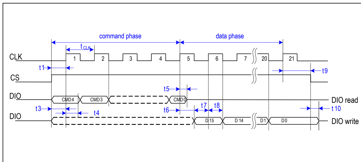
Figure 21: Timing Diagram in 3-Wire SSI R/W Mode
