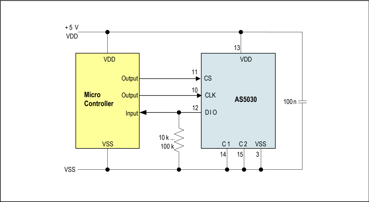
Figure 23: SSI Read-Only Serial Data Transmission
