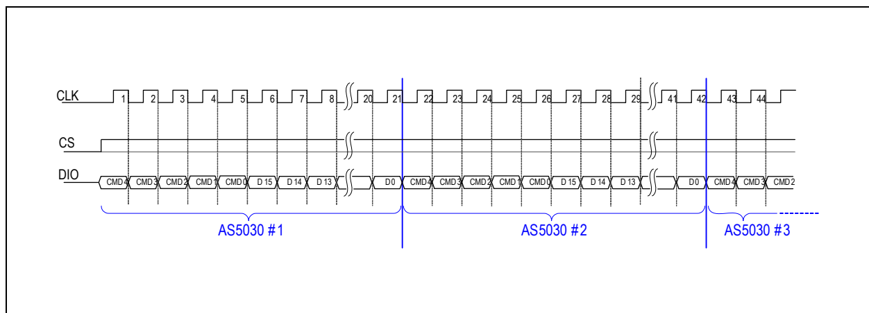
Figure 39: Timing Diagram in 3-Wire Daisy Chain Mode
