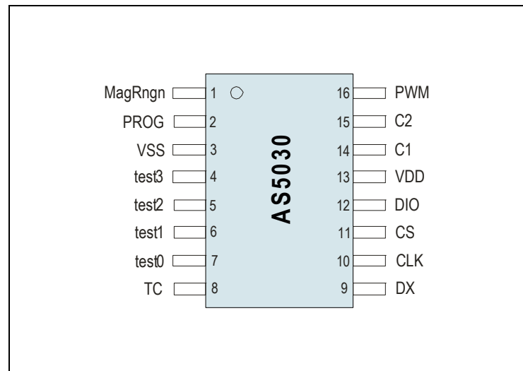
Figure 4: Pin Diagram (Top View)
