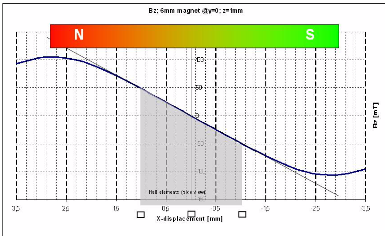
Figure 61: Bz Field Distribution Along the X-Axis of a 6mmØ Diametric Magnetized Magnet
