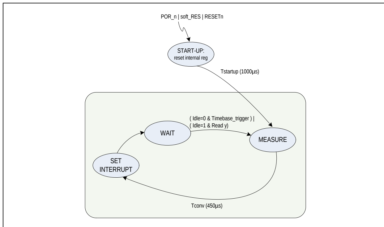
Figure 12: Readout Cycle Depending on Power Mode (idle bit)
