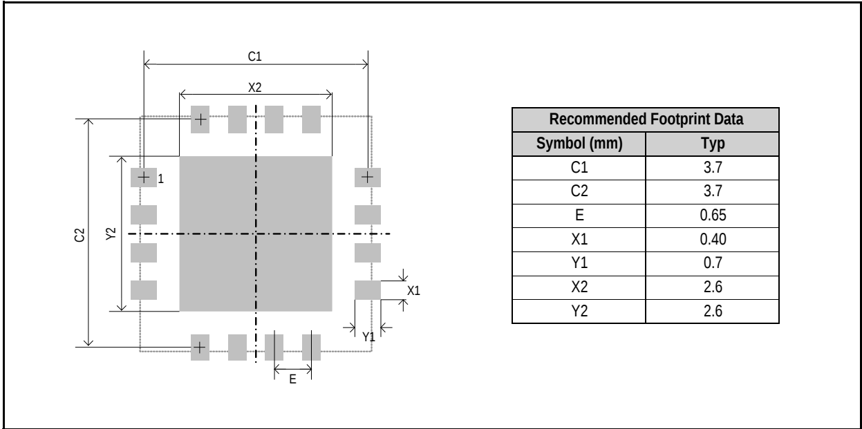
Figure 44: Footprint
