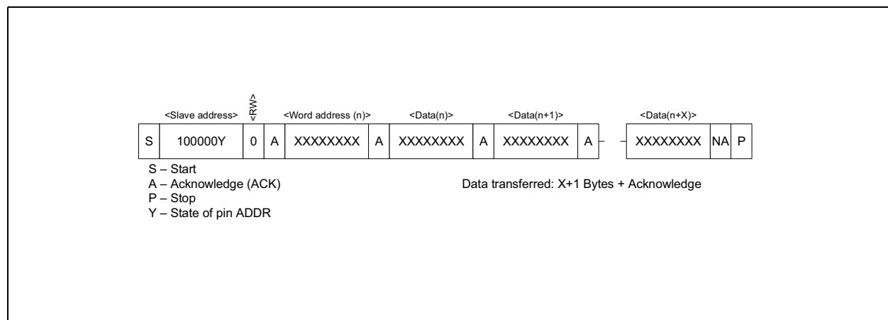
Figure 18: Data Write - Slave Receiver Mode
