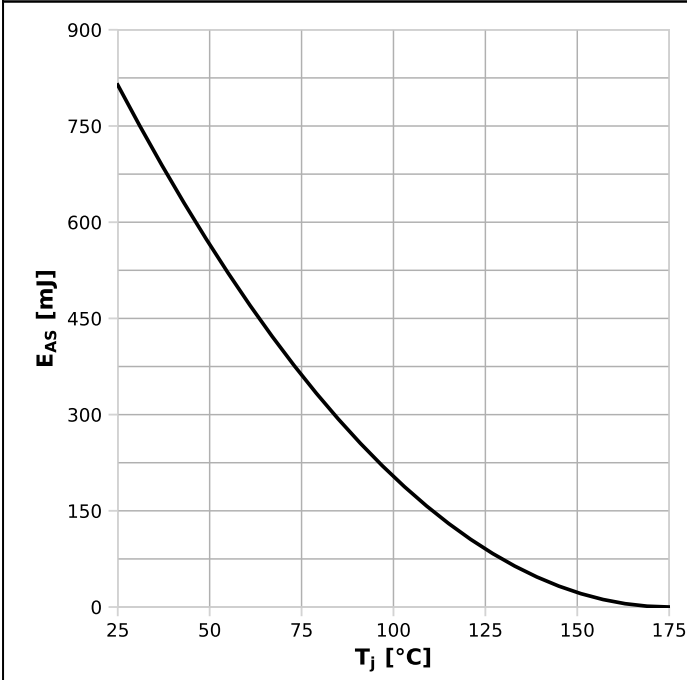
Diagram 13: Avalanche energy
