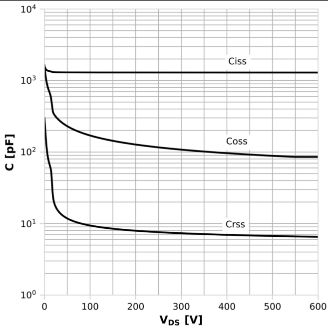
Diagram 15: Typ. capacitances
