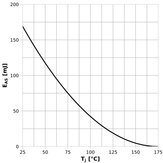
Diagram 13: Avalanche energy
