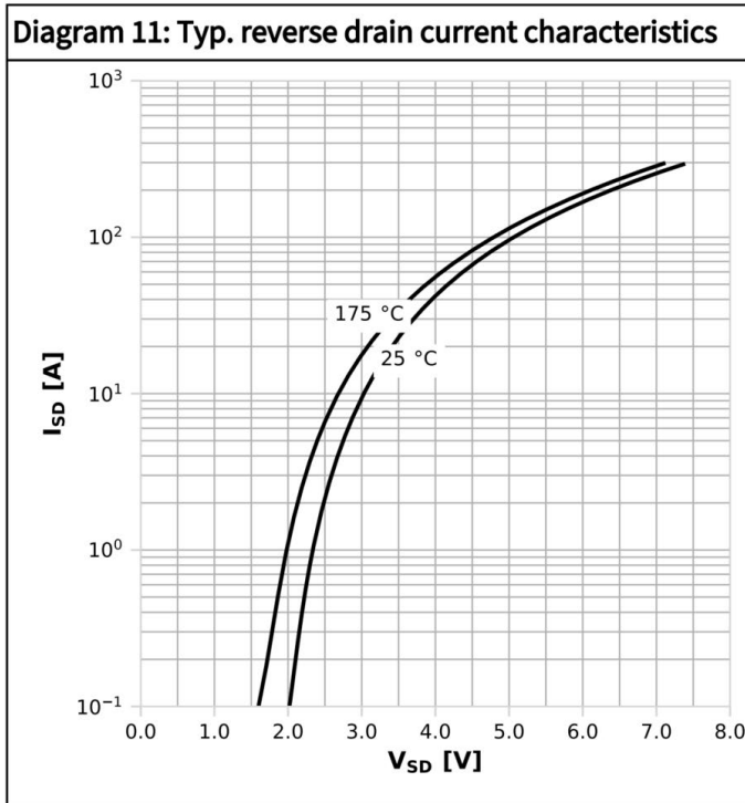
I_{SD}=f(V_{SD}); V_{GS}=0\text{ V}; \text{parameter: } T_j
