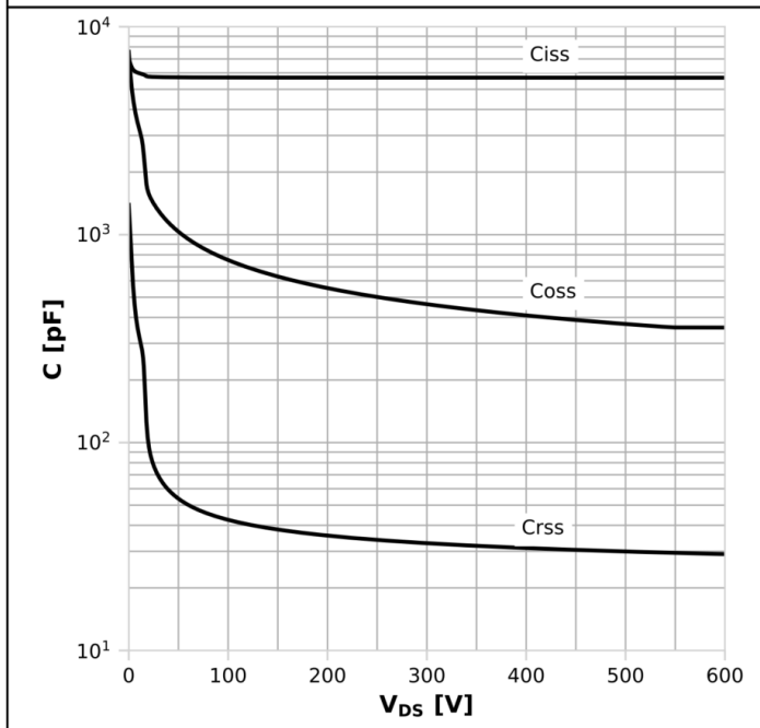
Diagram 15: Typ. capacitances
