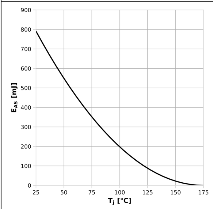
Diagram 13: Avalanche energy
