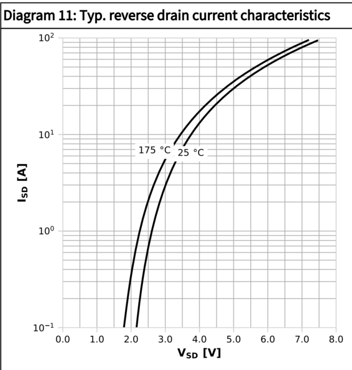
I_{SD}=f(V_{SD}); V_{GS}=0\text{ V}; \text{parameter: } T_j
