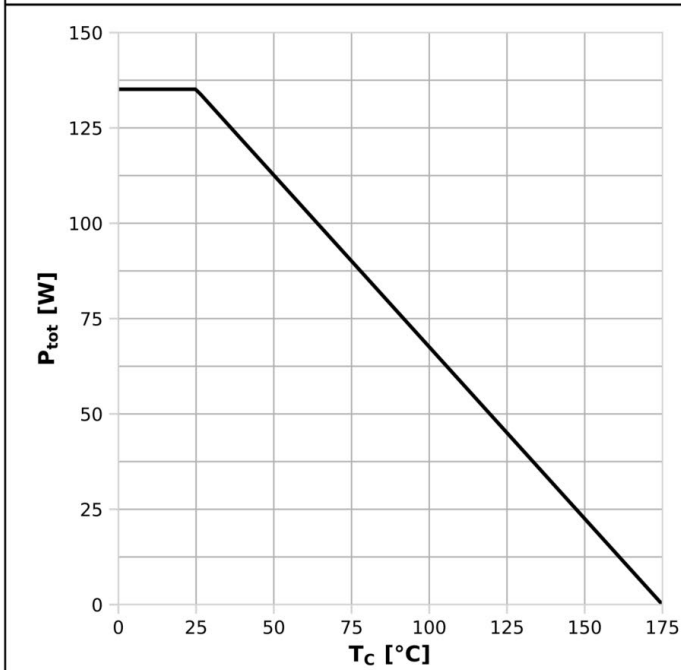
Diagram 1: Power dissipation
