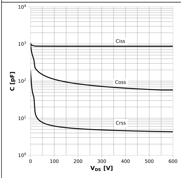
Diagram 15: Typ. capacitances
